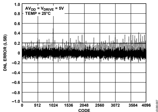
Figure 7. Typical DNL
