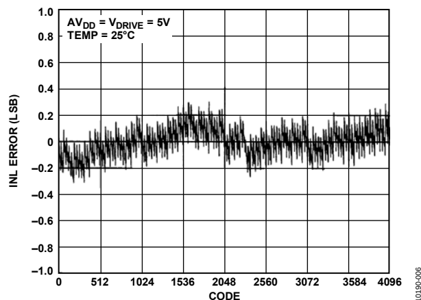
Figure 6. Typical INL
