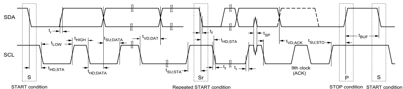
Figure 41. Timing Diagram
