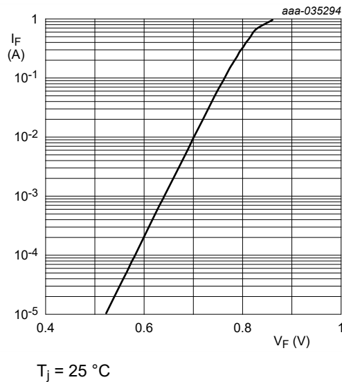
Fig. 6. Forward current as a function of forward voltage; typical values (HPZR-C7V0)
