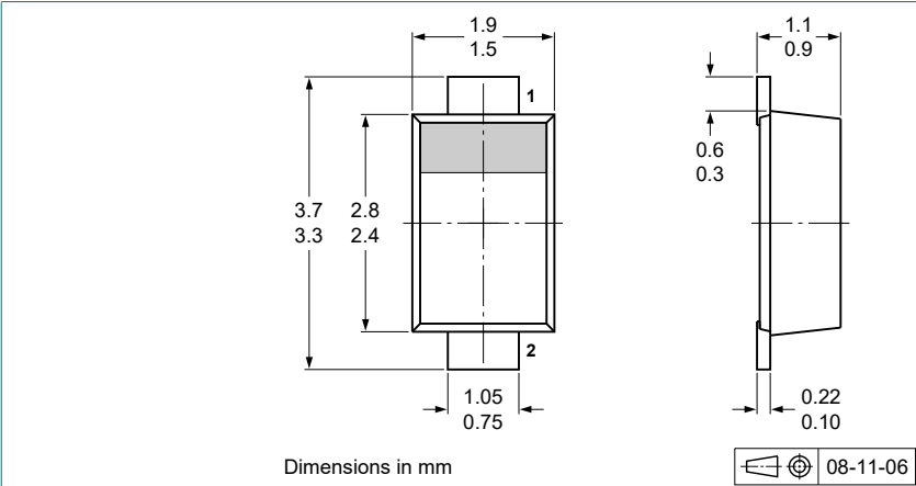
Fig. 10. Package outline CFP3 (SOD123W)
