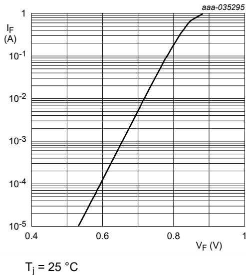
Fig. 7. Forward current as a function of forward voltage; typical values (HPZR-C8V2)
