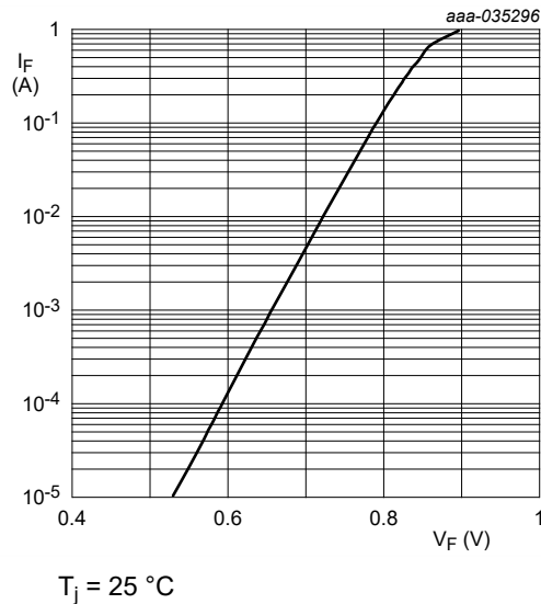
Fig. 8. Forward current as a function of forward voltage; typical values (HPZR-C68)
