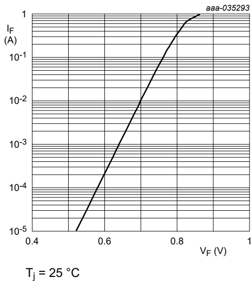
Fig. 5. Forward current as a function of forward voltage; typical values (HPZR-C5V6)
