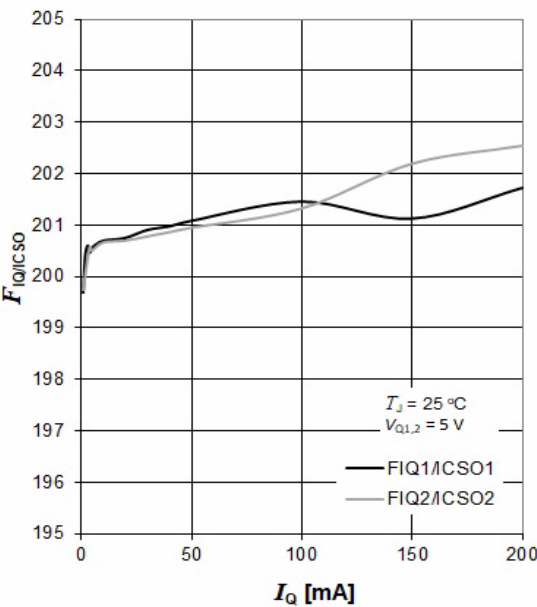
Current monitor factor F_{I_{Q}/I_{CSO\ 1,2,x}} versus output current I_{Q1,2}
