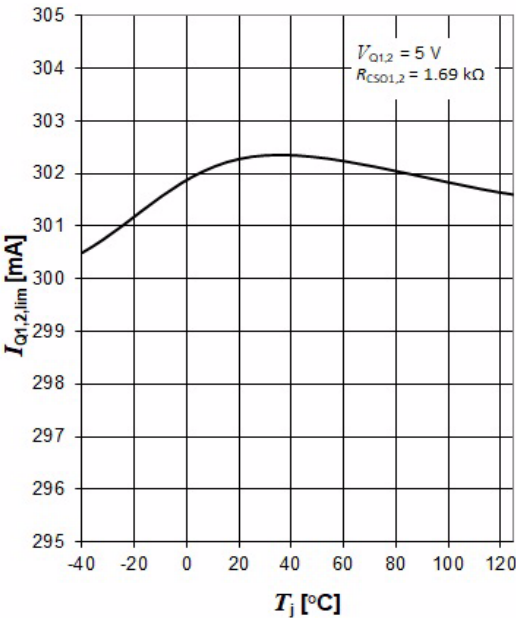
External current limitation I_{Q,lim1,2} versus junction temperature T_j
