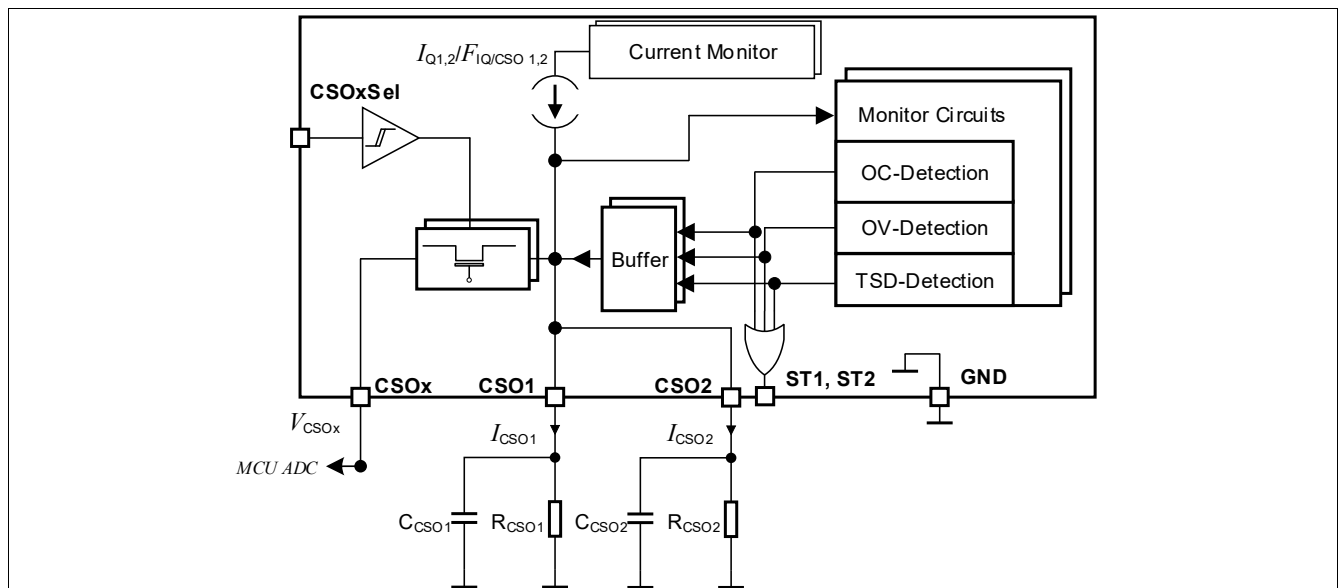
Figure 5 Functional block diagram current and protection monitor
