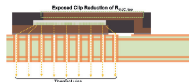
Source-Down PQFN 3.3x3.3 mm
