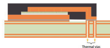
Drain-Down PQFN 3.3x3.3 mm
