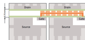
Source-Down - creepage distance
