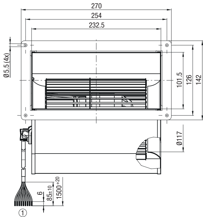
① Cable (halogen-free): BETrans ® GKW flex R, 9G 0.5 mm 2 , 9x crimped splices
