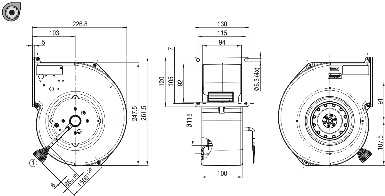
① Cable (halogen-free): BETrans ® GKW flex R, 9G 0.5 mm 2 , 9x crimped splices
