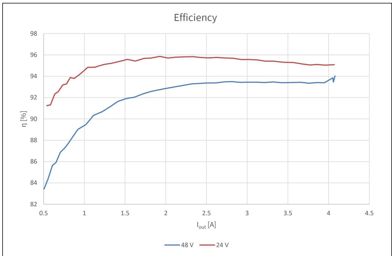
Figure 7 Efficiency at 12 V output in buck mode (R36 has been bridged)
