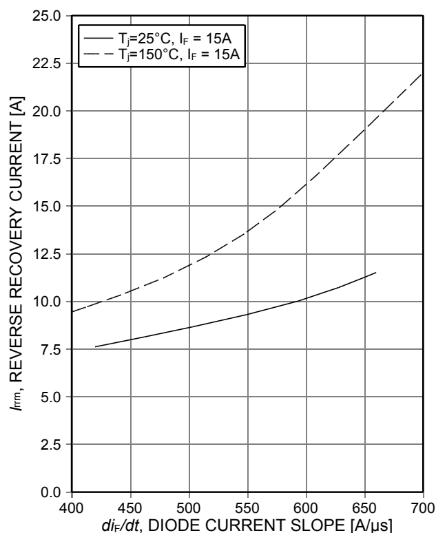
Figure 21. Typical peak reverse recovery current as a function of diode current slope ( V_R = 400\text{V} )
