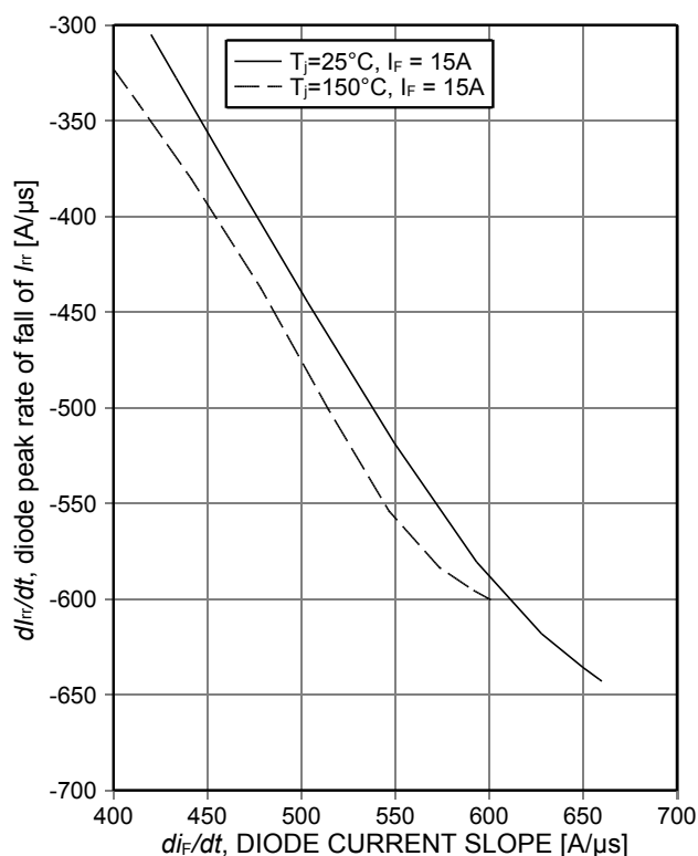
Figure 22. Typical diode peak rate of fall of reverse recovery current as a function of diode current slope ( V_R = 400\text{V} )
