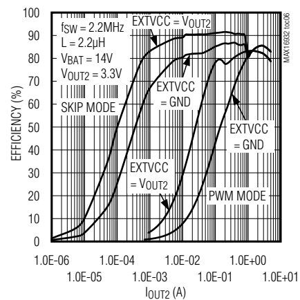
BUCK2 EFFICIENCY
