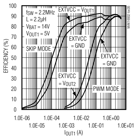
BUCK1 EFFICIENCY
