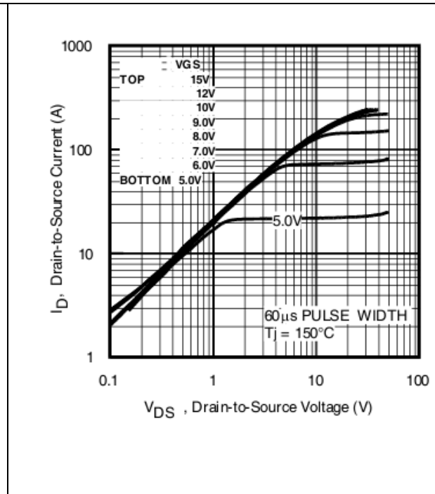
Figure 3 Typical Output Characteristics
