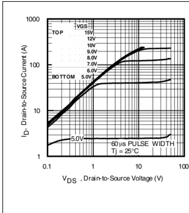
Figure 2 Typical Output Characteristics
