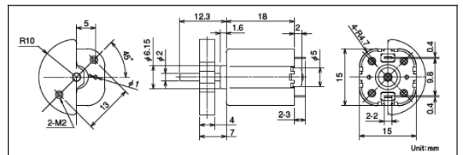
SE15H0STTS product drawing
