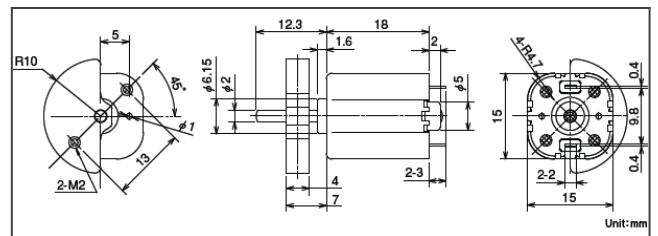
SE15H0STTS Model Product Drawing
