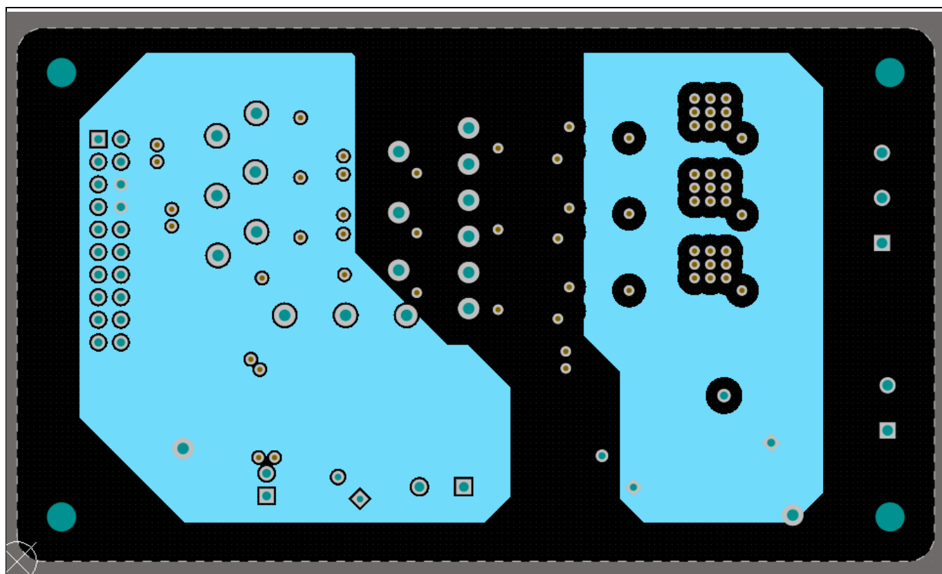
Figure 22 Power inverter board layout (Middle layer- layer 3)
