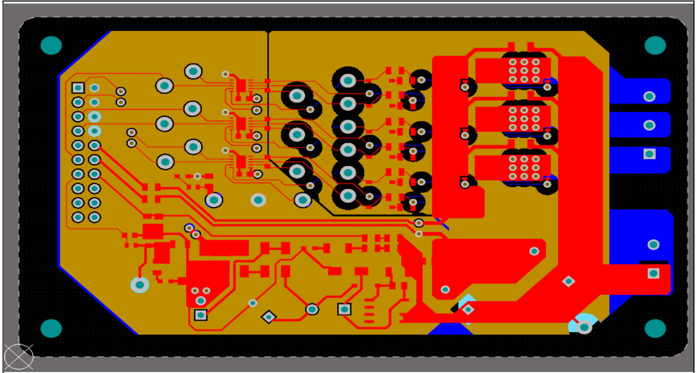
Figure 19 Power inverter board layout (All 4 layers together)
