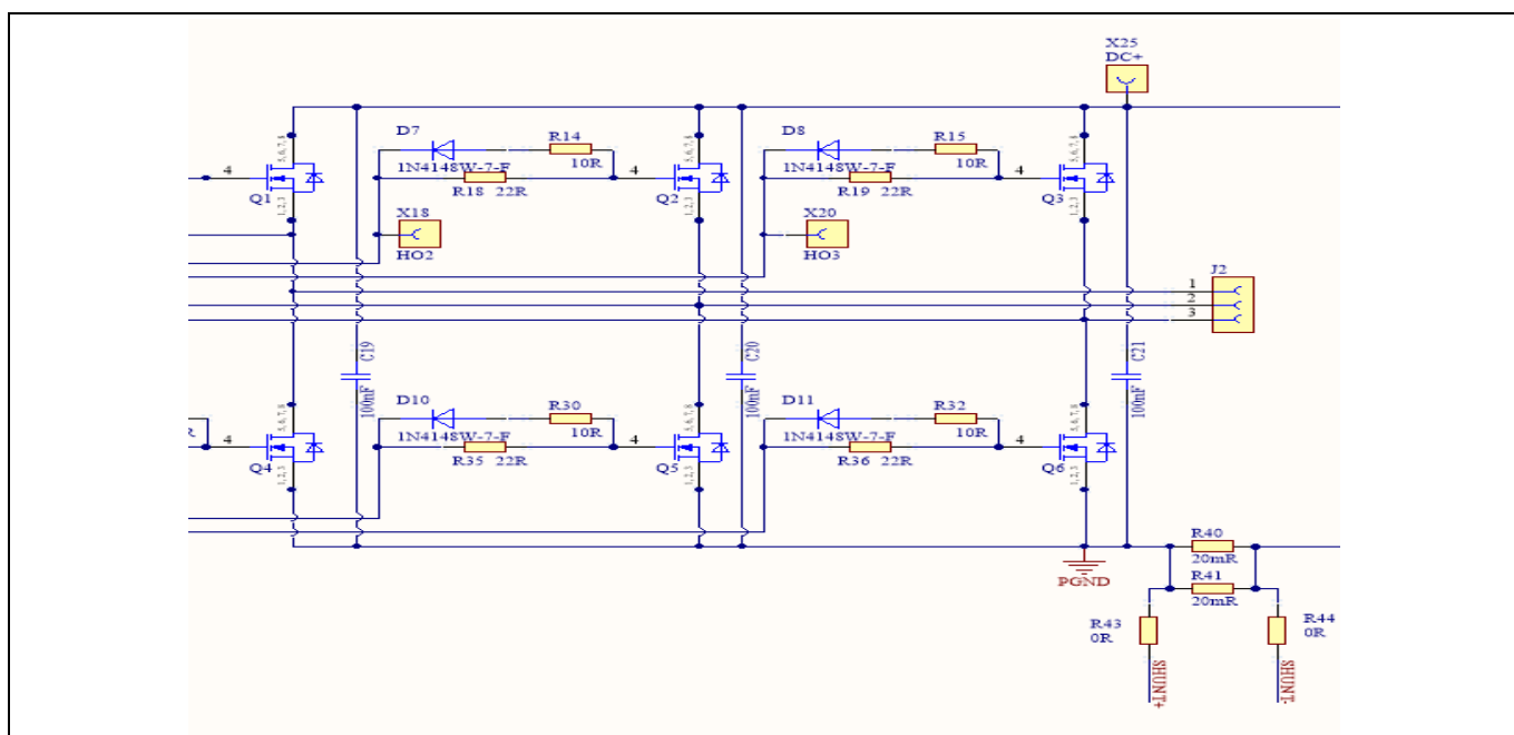
Figure 15 The diagram of the BSC074N15NS5 based inverter section with single shunt current sense
