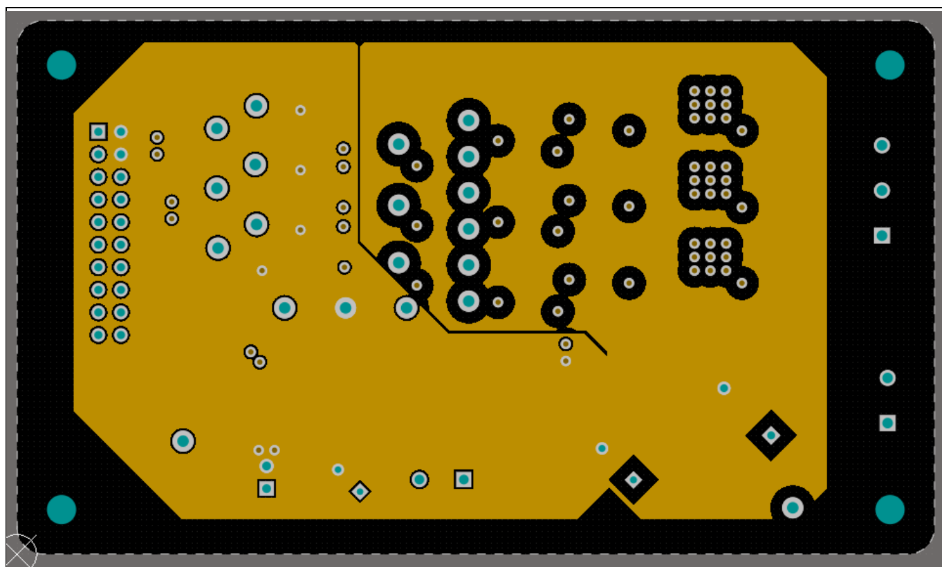
Figure 21 Power inverter board layout (Middle layer- layer 2)
