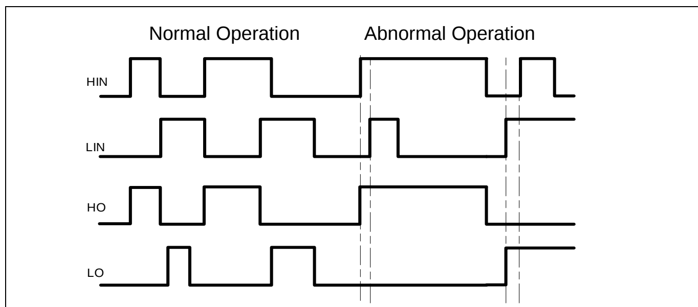
Figure 10 Illustration of shoot-through protection circuitry
