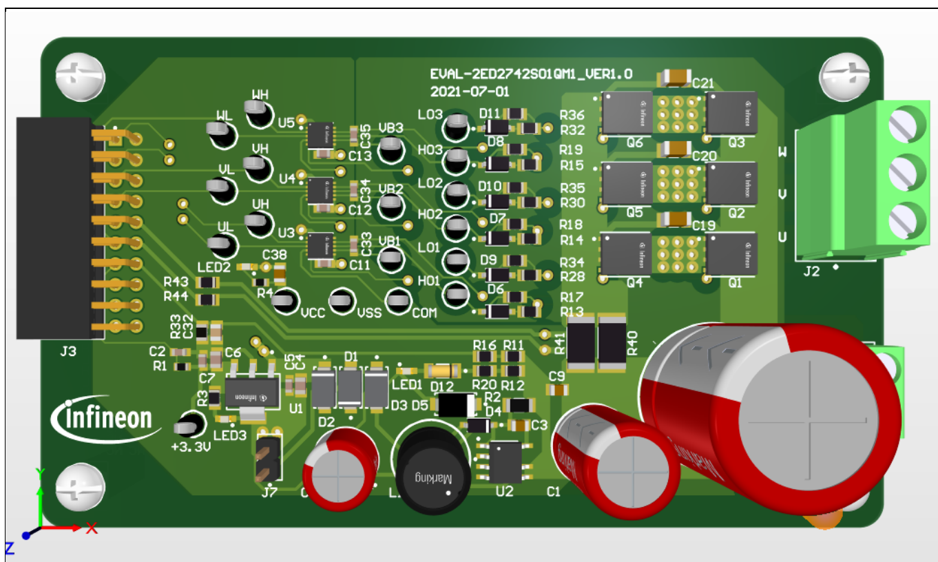
Figure 24 Power inverter assembled board
