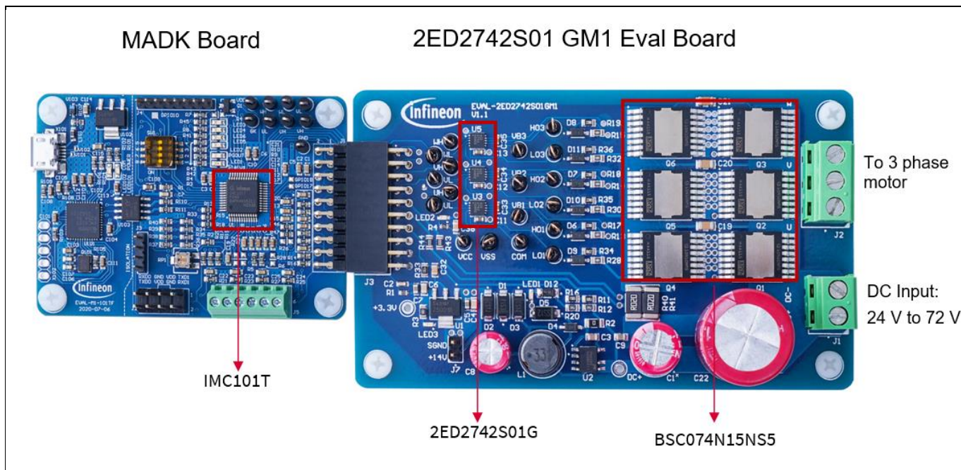
Figure 2 Functional blocks of EVAL-2ED2742S01 GM1 BPA Evaluation Kit (top view) w/o heatsink
