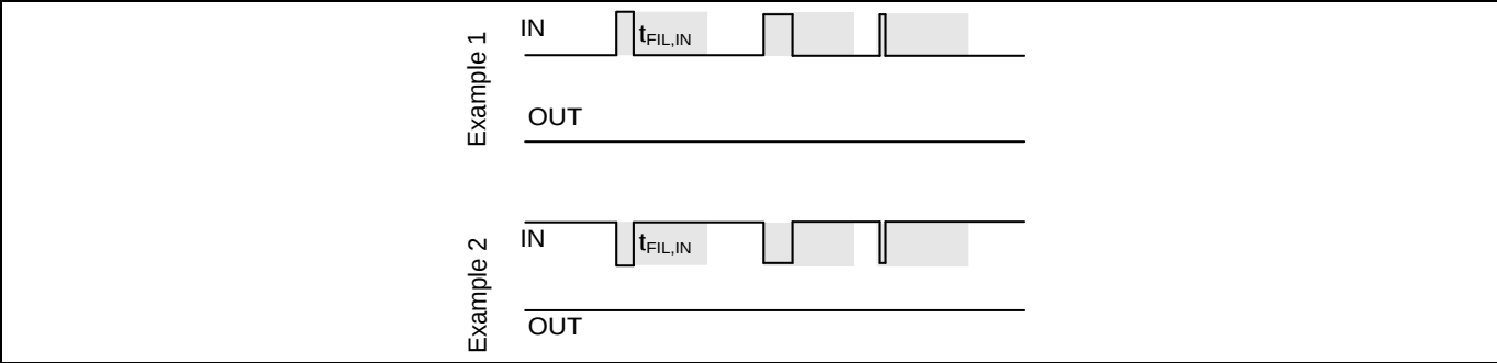
Figure 11 Noise Rejecting Input Filters
