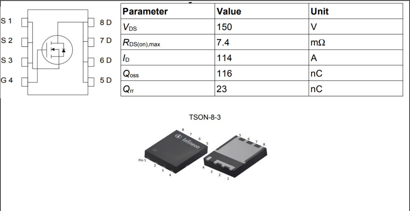
Figure 12 Key features of BSC074N15NS5
