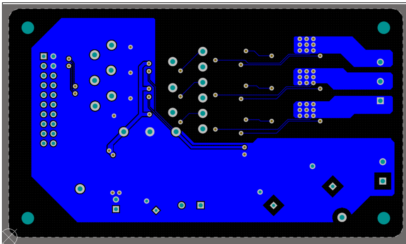
Figure 23 Power inverter board layout (bottom view- layer 4)
