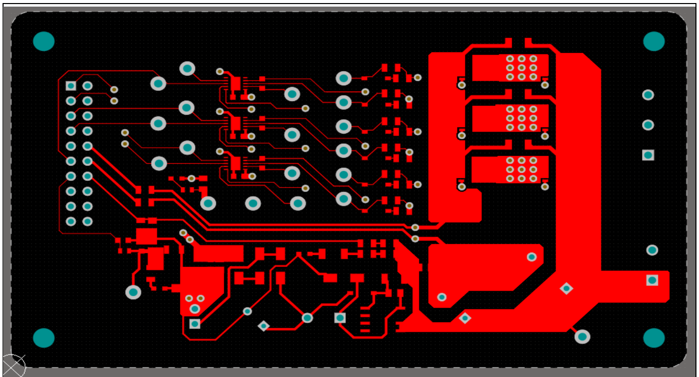
Figure 20 Power inverter board layout (Top view- layer 1)
