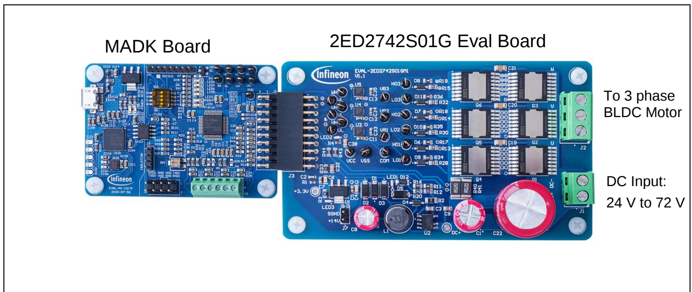
Figure 25 System setup for running a BLDC motor
