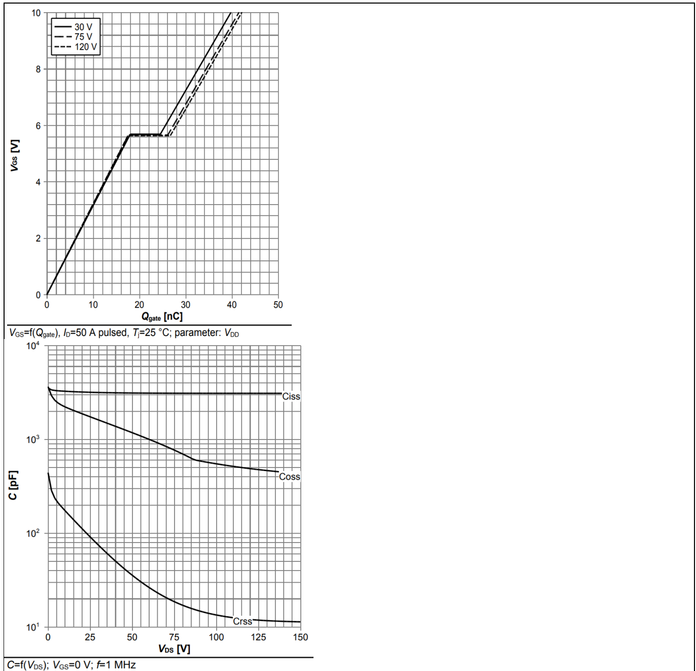
Figure 13 BSC074N15NS5 typical characteristics
