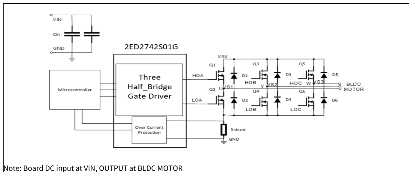
Figure 1 Simplified application block diagram of EVAL-2ED2742S01 GM1
