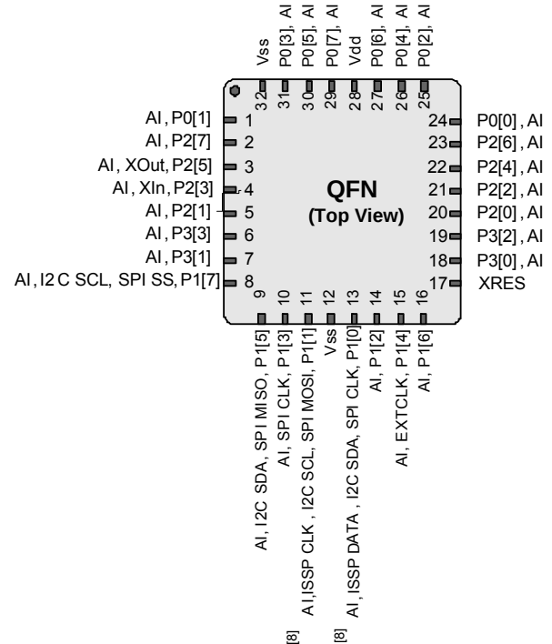
Figure 3. CY8C24193
