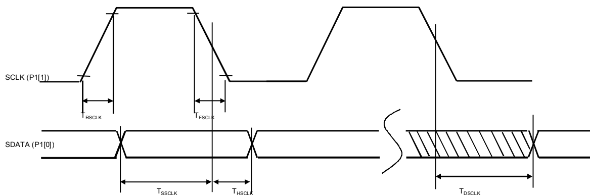
Figure 18. AC Waveform
