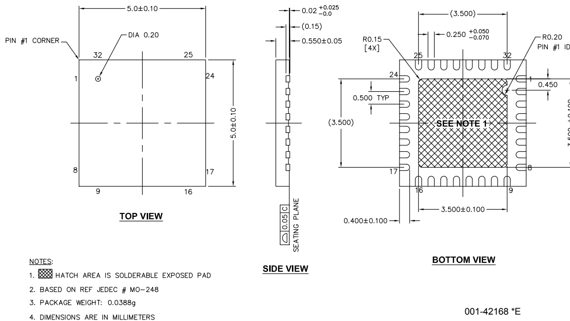
Figure 24. 32-pin QFN ( 5 \times 5 \times 0.55 mm) LQ32 3.5 \times 3.5 E-Pad (Sawn) Package Outline, 001-42168
