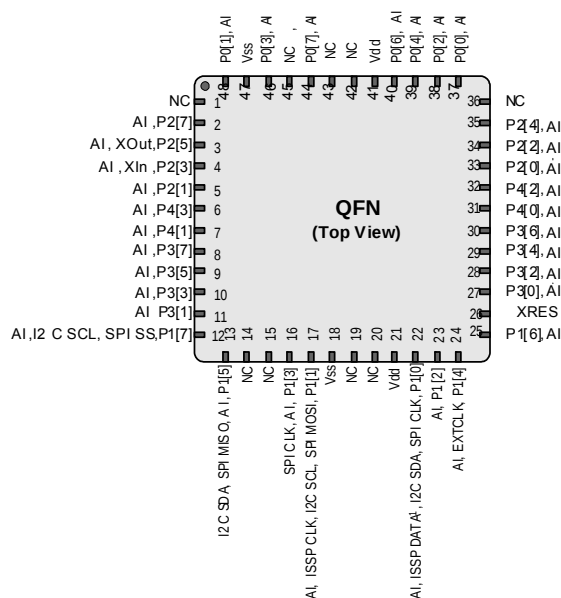
Figure 5. CY8C24393, CY8C24693 Device
