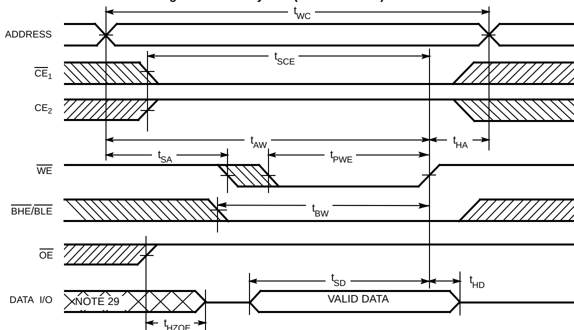
Figure 8. Write Cycle 2 ( \overline{CE}_1 or CE_2 Controlled) [26, 27, 28, 29]
