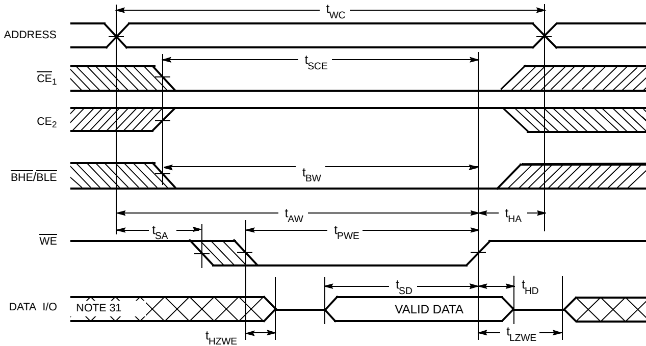
Figure 10. Write Cycle 4 ( \overline{BHE/BLER} Controlled, \overline{OE} LOW) [30, 32]
