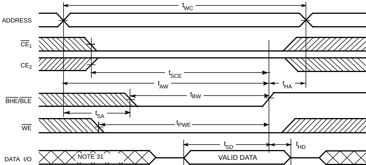
Figure 10. Write Cycle 4 ( \overline{BHE/BLER} Controlled, \overline{OE} LOW) [30, 32]
