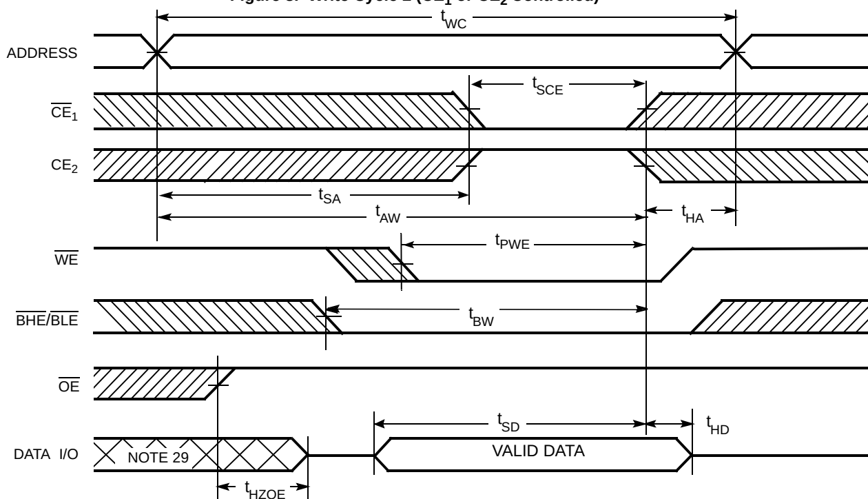
Figure 8. Write Cycle 2 ( \overline{CE}_1 or CE_2 Controlled) [26, 27, 28, 29]
