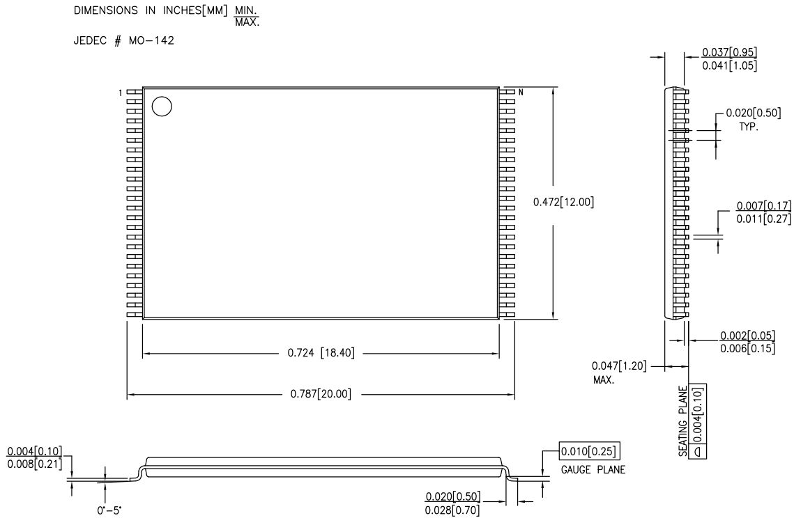
Figure 12. 48-pin TSOP I (12 × 18.4 × 1 mm) Z48A Package Outline, 51-85183
