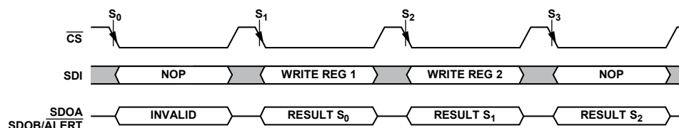
Figure 44. Register Write
