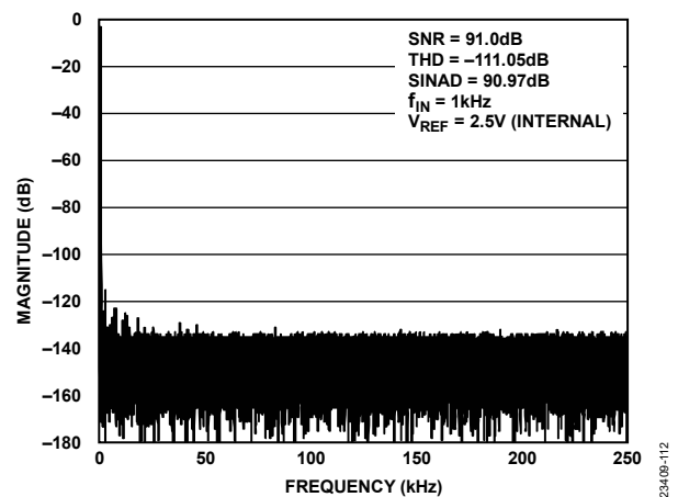
Figure 12. AD4681 FFT, V_{REF} = 2.5 V Internal
