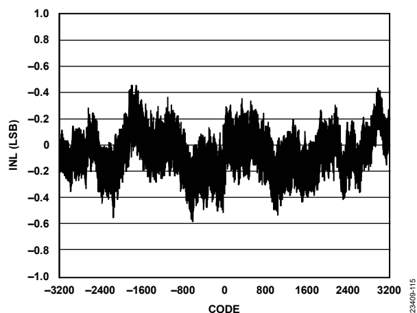
Figure 15. INL Error
