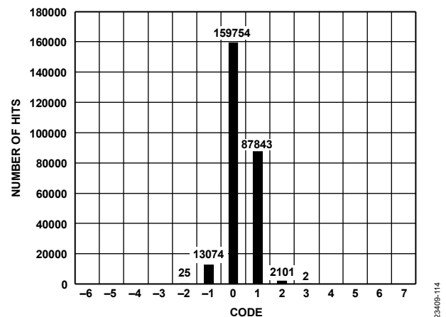
Figure 14. DC Histogram Codes at Code Center
