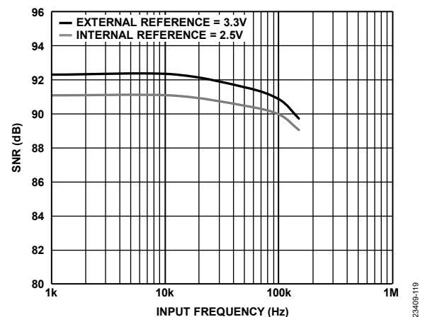
Figure 19. AD4680 SNR vs. Input Frequency
