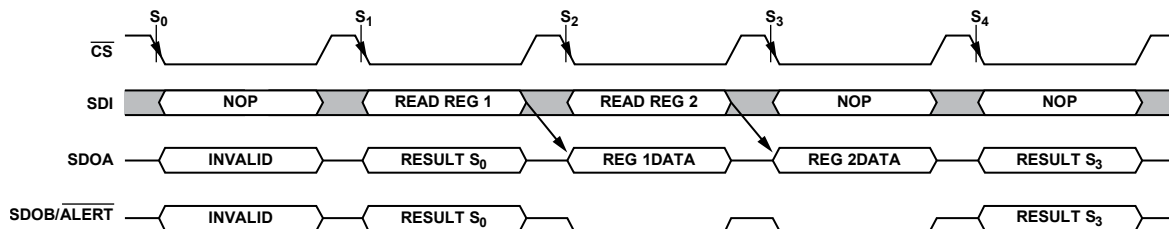
Figure 43. Register Read
