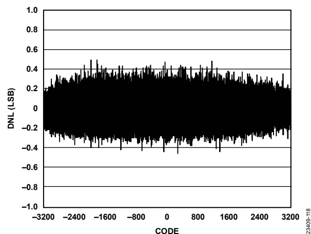
Figure 18. DNL Error
