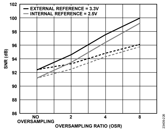
Figure 26. AD4680 SNR vs. Oversampling Ratio, Oversampling Mode
