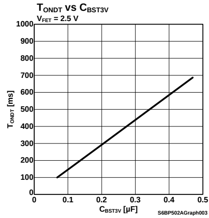
Figure 10-5 High-side FET On-duration Time vs C_{BST3V}
