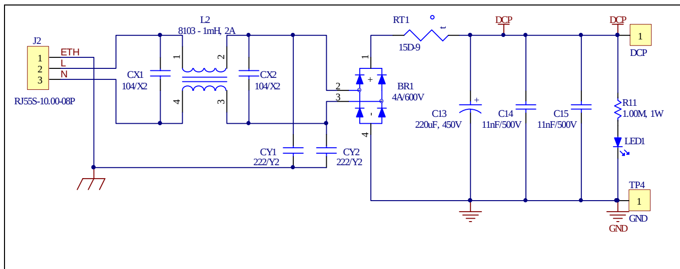
Figure 18 Schematic for EMI filter and AC/DC section of the EVAL-M1-IM240-A evaluation board
