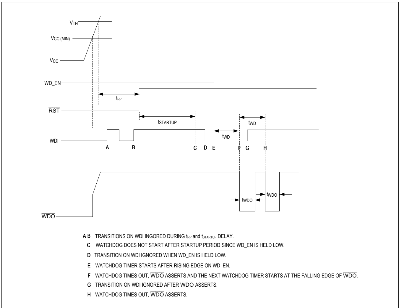
Figure 3. Watchdog Timing Characteristics with \overline{WD\_EN} Active After Startup Time
