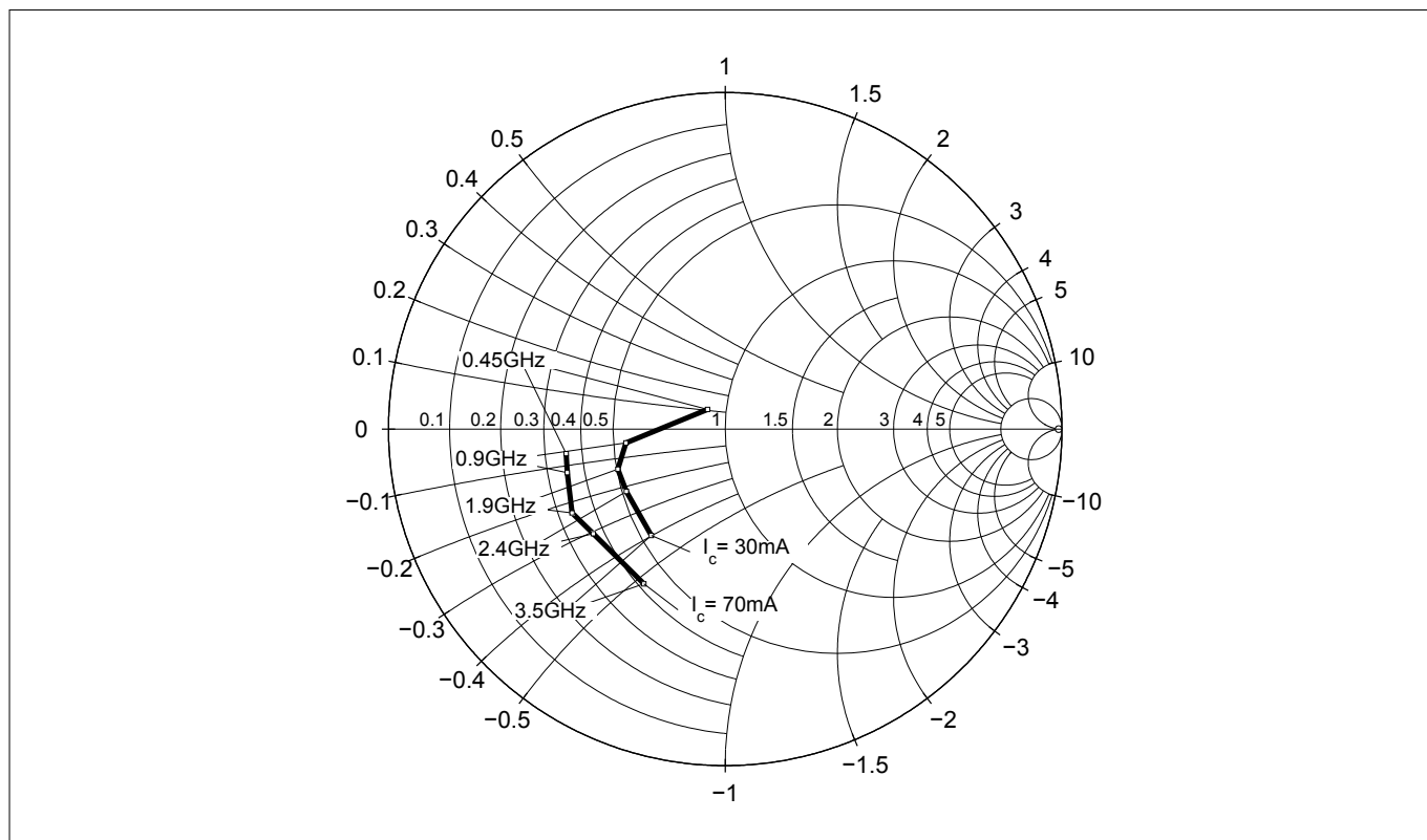
Figure 15 Source impedance for minimum noise figure Z_{s,opt} = f(f) , V_{CE} = 3\text{ V} , I_C = 30 / 70\text{ mA}
