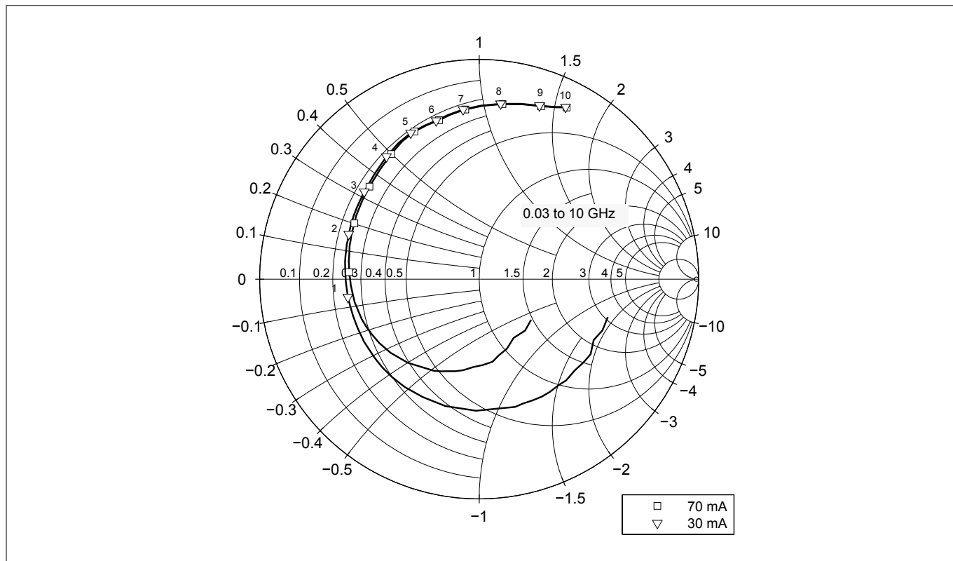
Figure 14 Input reflection coefficient S_{11} = f(f) , V_{CE} = 3\text{ V} , I_C = 30 / 70\text{ mA}
