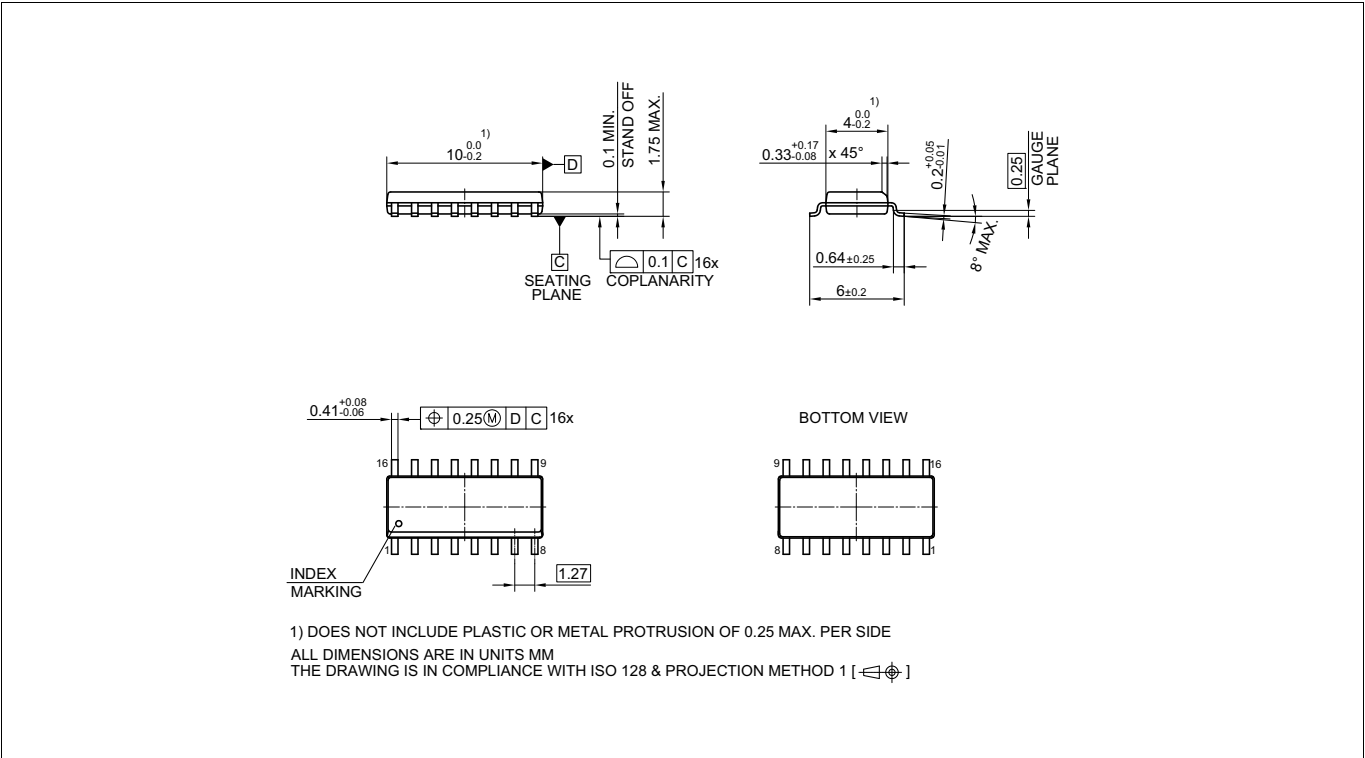
Figure 15 PG-DSO-16-11 outline
