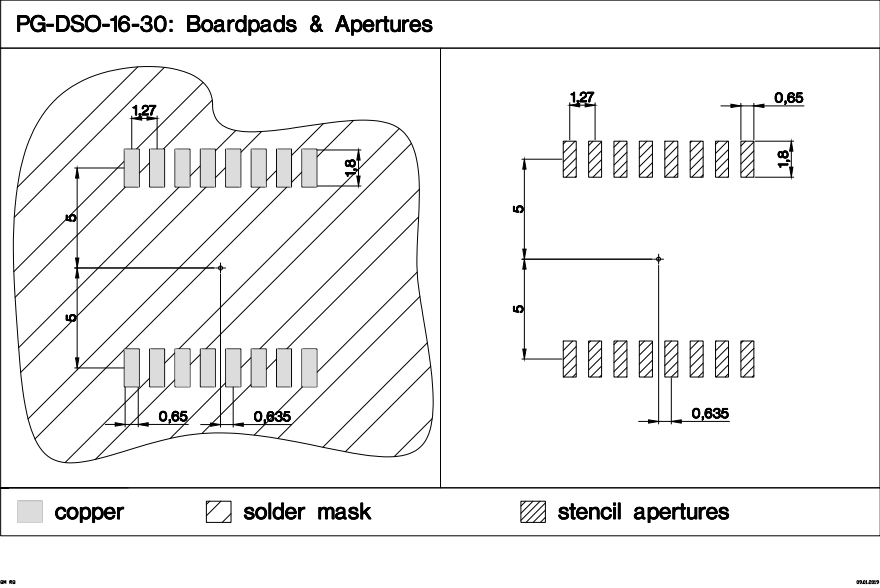
Figure 19 PG-DSO-16-30 footprint
