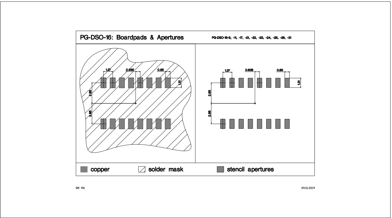
Figure 16 PG-DSO-16-11 footprint
