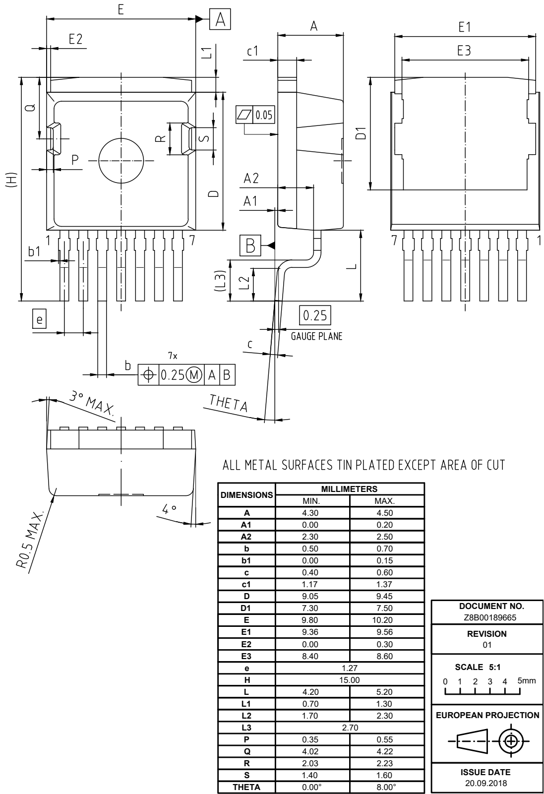
Figure 1 Outline PG-T0263-7-11, dimensions in mm
