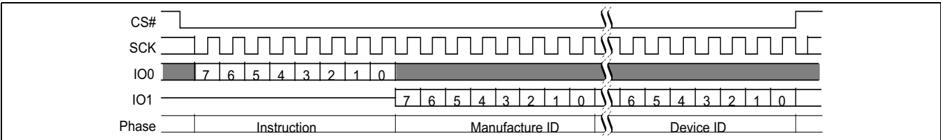
Figure 31 READ_ID (90h) command sequence
