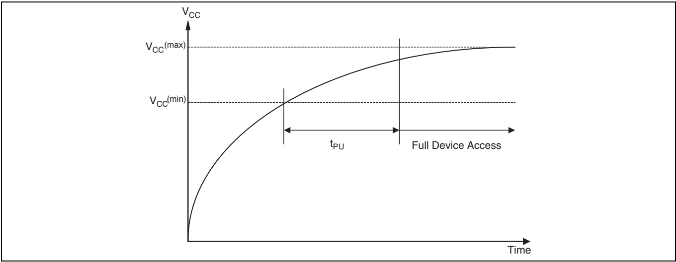
Figure 13 Power-up
