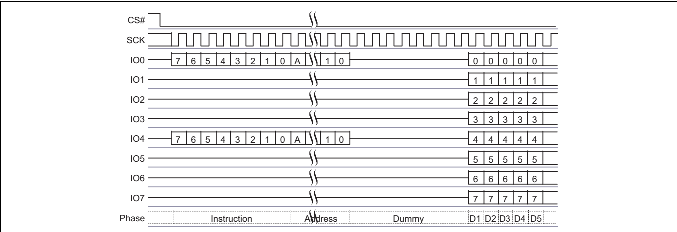
Figure 55 Dual-Quad, Quad Output Read (QOR 6Bh or 4QOR 6Ch) command sequence
