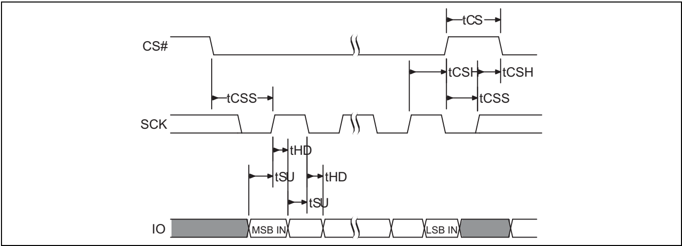
Figure 24 SPI DDR input timing
