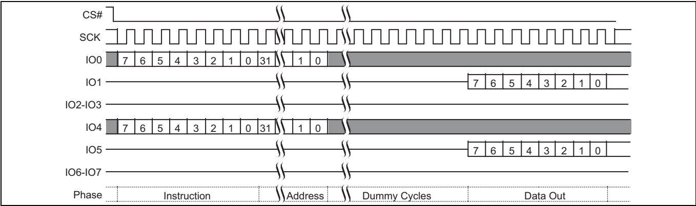
Figure 46 ECC Status Register Read command sequence
