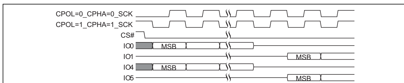
Figure 2 Dual-quad SPI SDR modes supported
