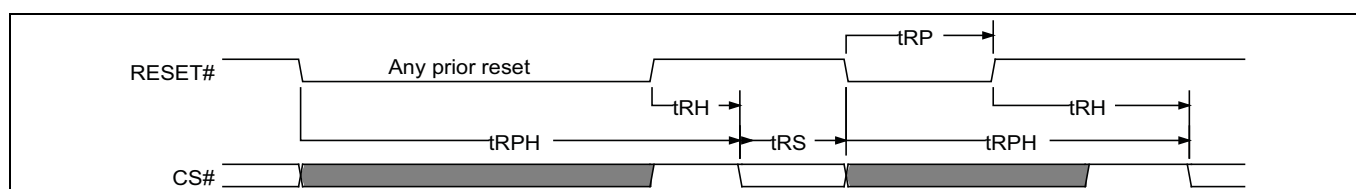
Figure 21 Hardware reset
