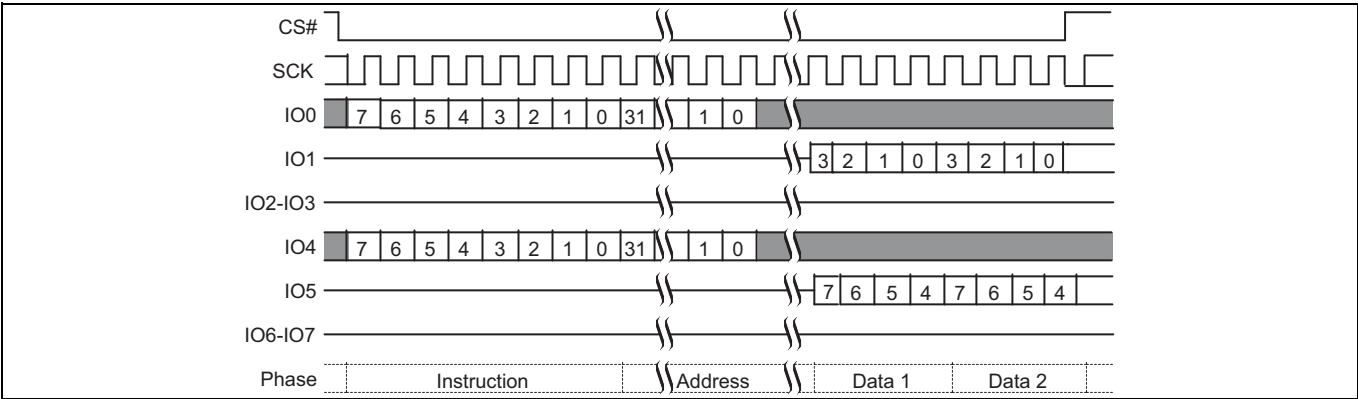
Figure 6 Dual-Quad Single bit Wide I/O command without latency
