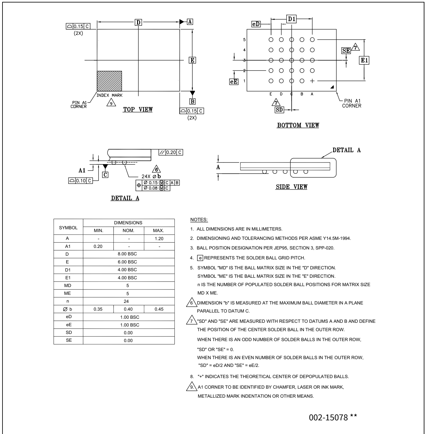
Figure 28 24-ball FBGA (8.0 × 6.0 × 1.2 mm) package outline (PG-TFBGA-24), 002-15078
