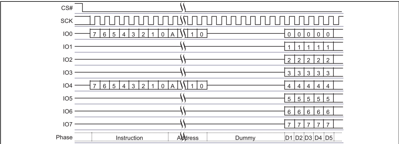
Figure 8 Dual-Quad, Quad Output Read command
