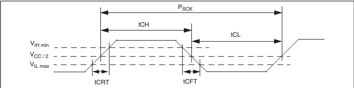
Figure 22 Clock timing
