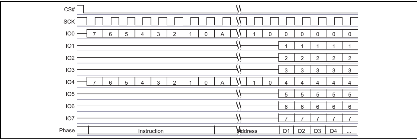
Figure 61 Dual-Quad, Quad Page Program command sequence
