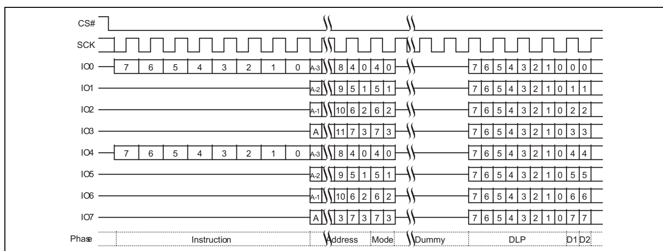
Figure 58 Dual-Quad SPI DDR Quad I/O Read Initial Access
