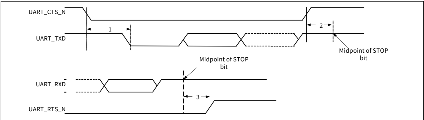
Figure 11 UART timing
