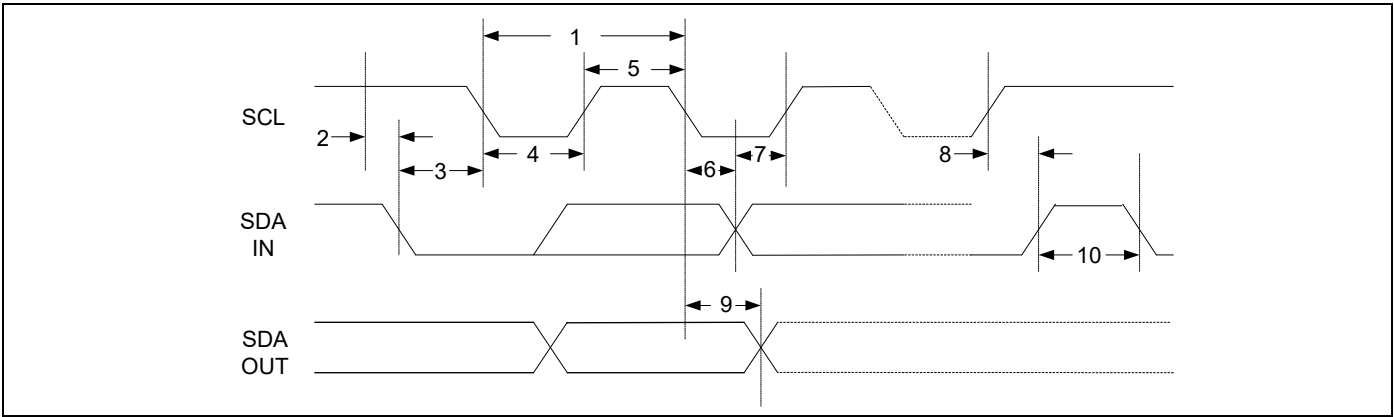
Figure 16 BSC interface timing diagram
