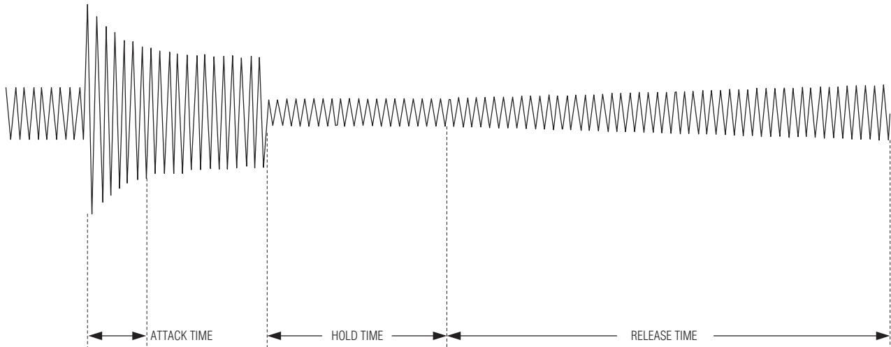
Figure 12. AGC Timing
