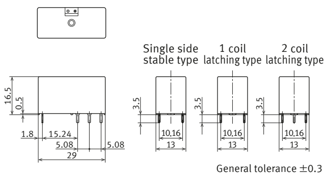
External dimensions
