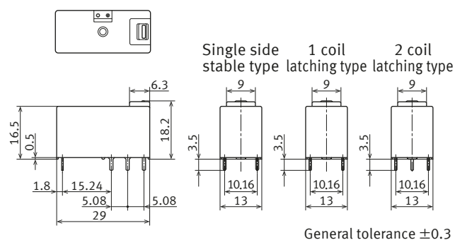
External dimensions
