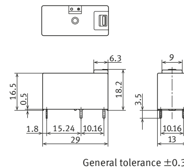
External dimensions
