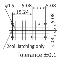
Recommended PC board pattern ( BOTTOM VIEW )
