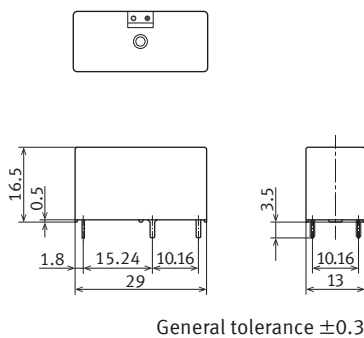
External dimensions
