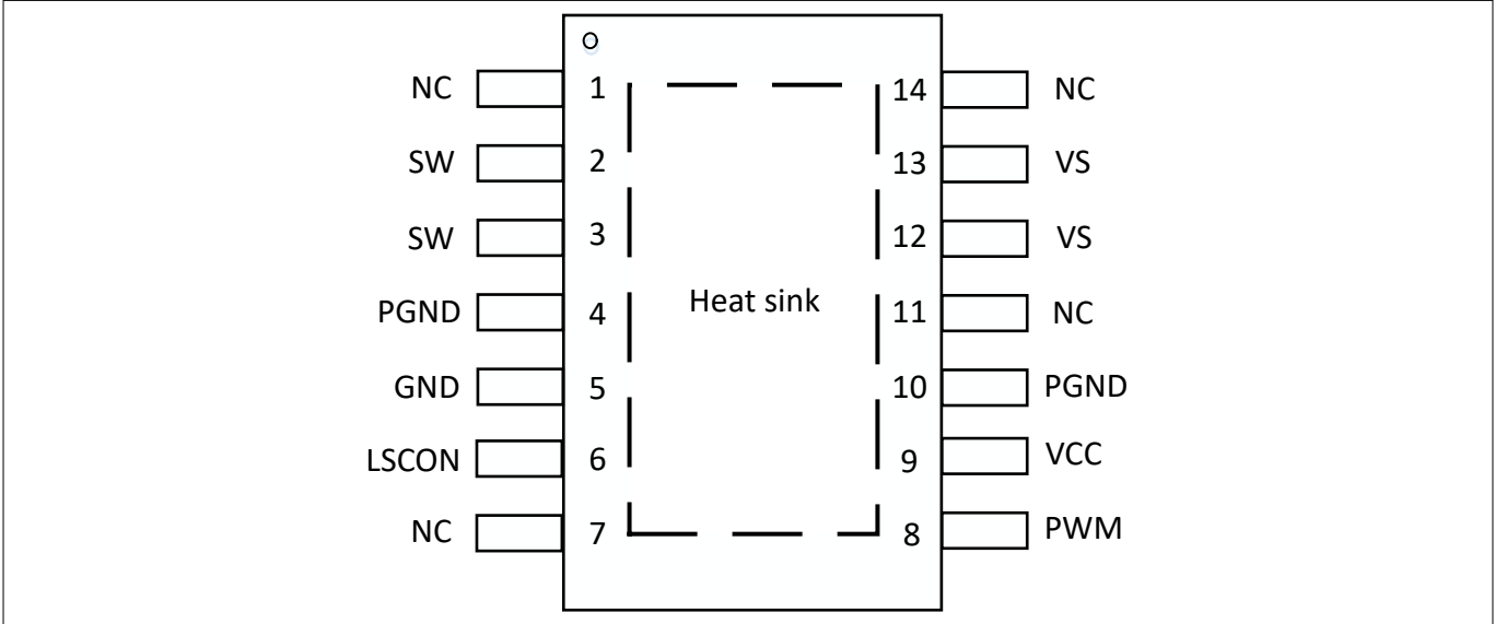
Figure 2 Pin configuration
