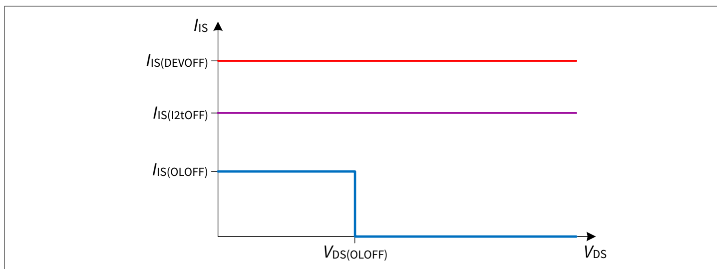
Figure 47 I_{IS} in OFF state
