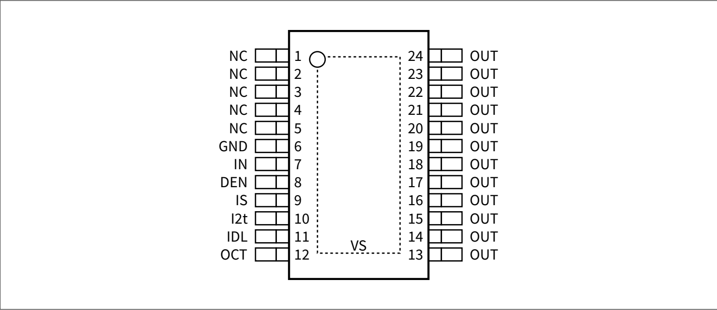
Figure 3 Pin configuration
