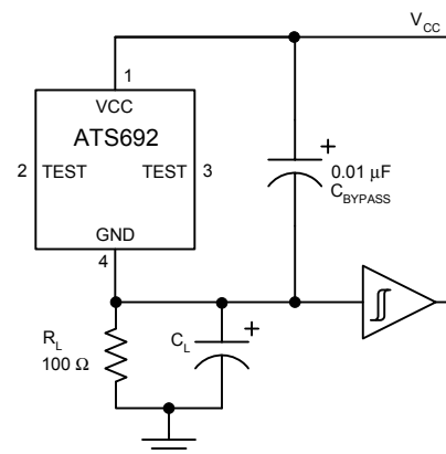
Figure 8. Typical application circuit
