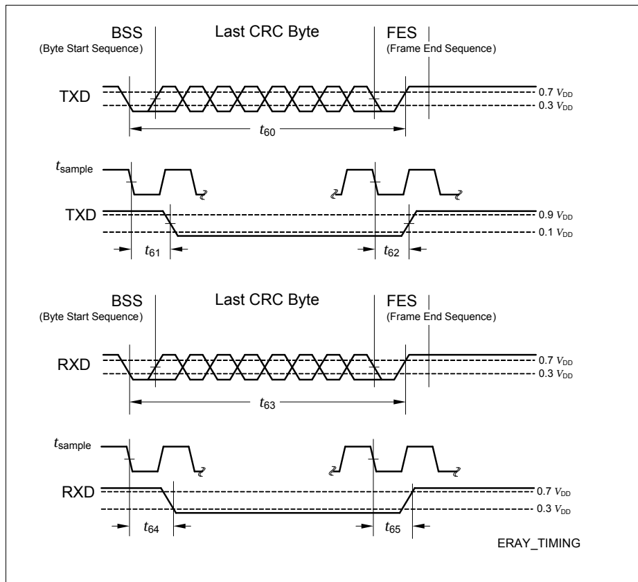
Figure 23 ERAY Timing
