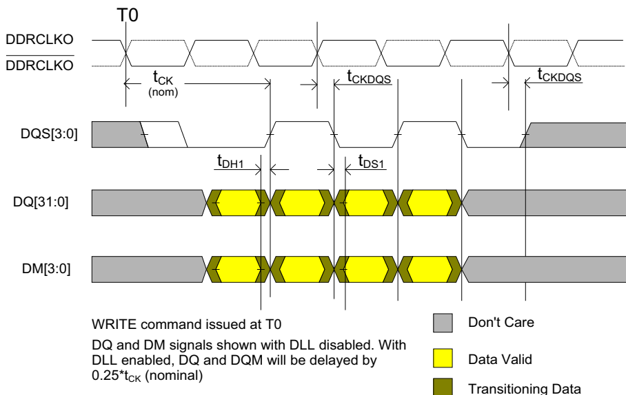
Figure 31 Signal Relationship for DDR writes
