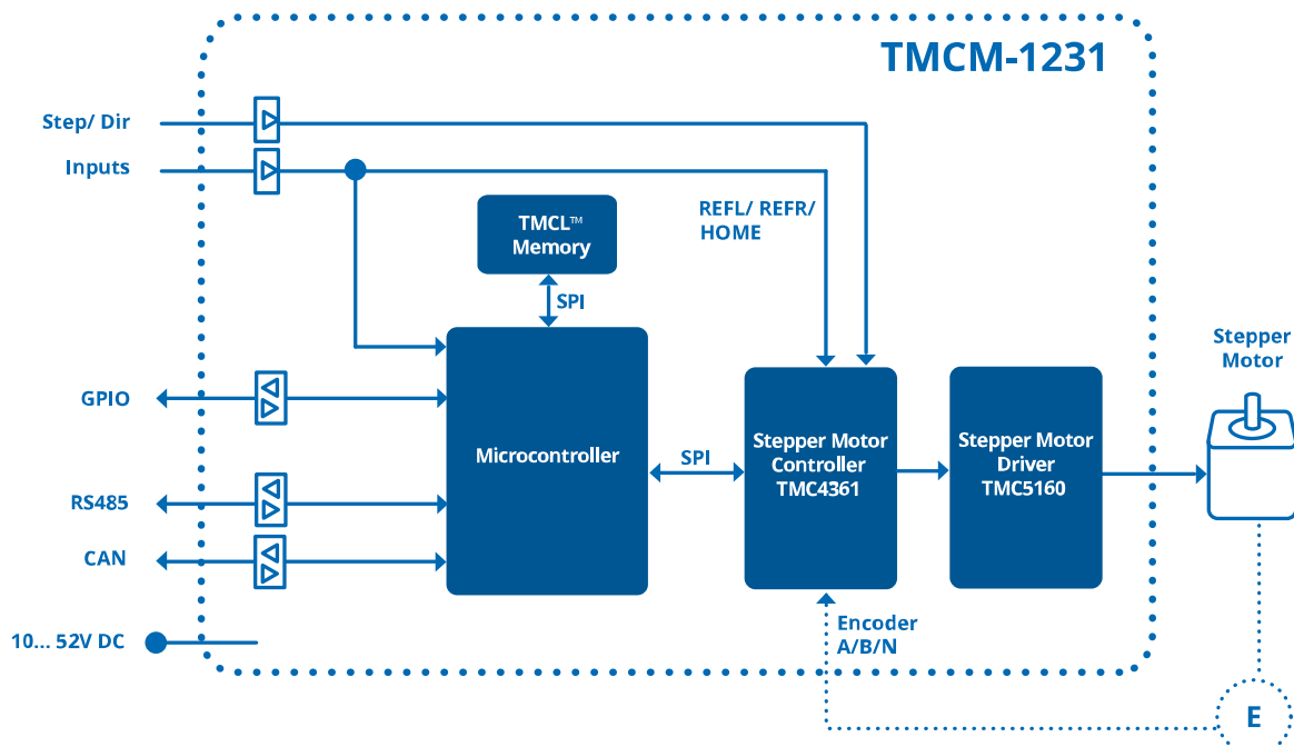
Figure 7: TMC-1231 block diagram
