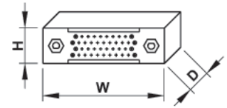
BODY CONNECTOR DIMENSIONS
