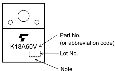
Fig. 7.1 Marking
