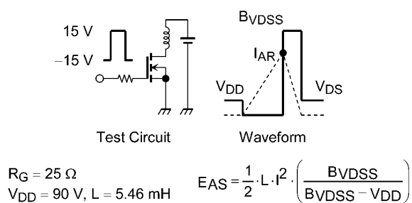
Fig. 8.16 Test Circuit/Waveform
