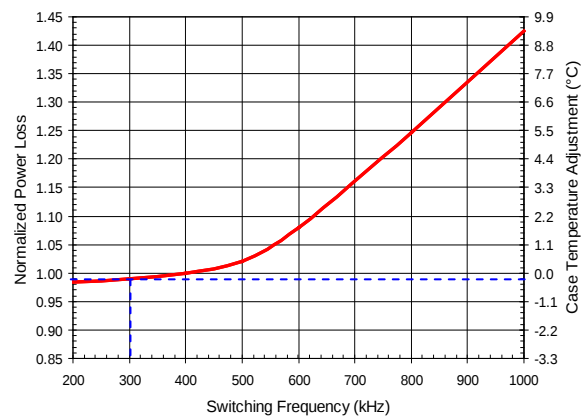
Figure 16: Normalized Power Loss vs. Switching Frequency
