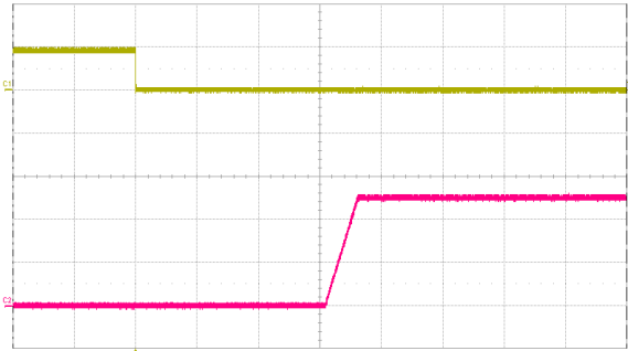
Fig. 9: Turn-on transient at full rated load current (resistive) with C_{out} 10 \mu F tantalum + 1 \mu F ceramic at V_{in} = 48 V, triggered via ON/OFF pin. Top trace: ON/OFF signal (5 V/div.). Bottom trace: output voltage (2 V/div.). Time scale: 20 ms/div.
