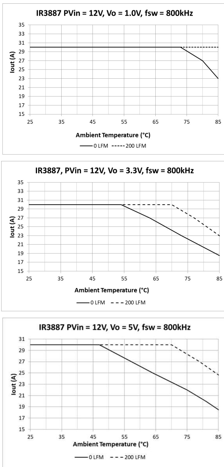
Figure 4 Thermal de-rating curves, P_{Vin} = 12\text{ V} , V_{out} = 1.0\text{ V}/3.3\text{ V}/5\text{ V} , f_{sw} = 800\text{ kHz} , VCC = Internal LDO
