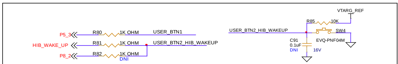
Figure 46 User buttons
