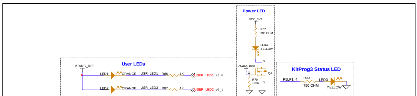
Figure 32 LEDs
