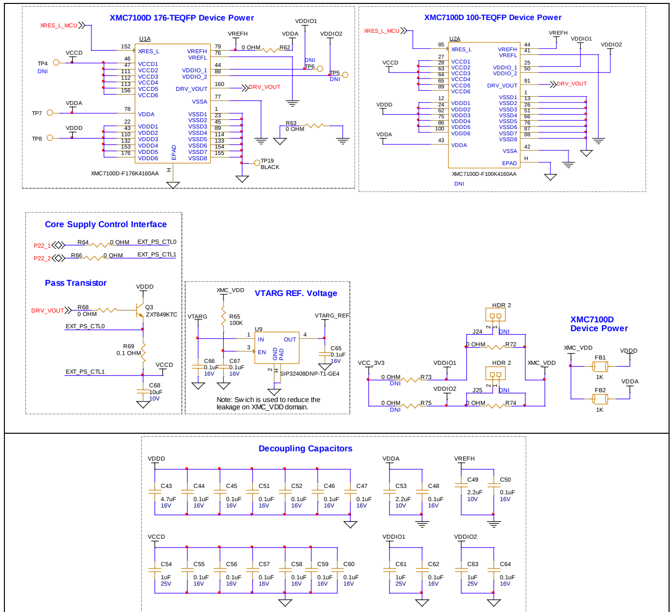
Figure 17 XMC7100D
