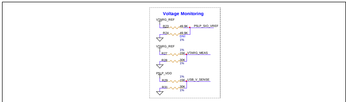
Figure 24 Voltage monitoring
