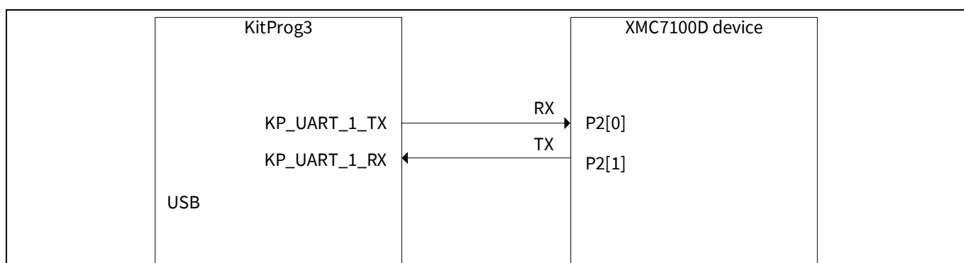
Figure 15 UART connection between KitProg3 and XMC7100D
