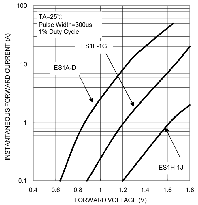
FIG. 2- TYPICAL INSTANTANEOUS FORWARD CHARACTERISTICS
