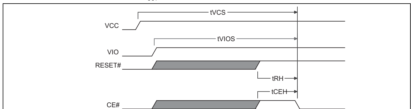
Figure 15 Power-Up diagram
