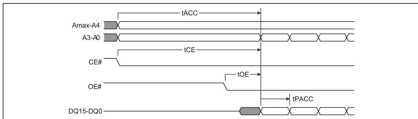
Figure 19 Page read timing diagram [92]
