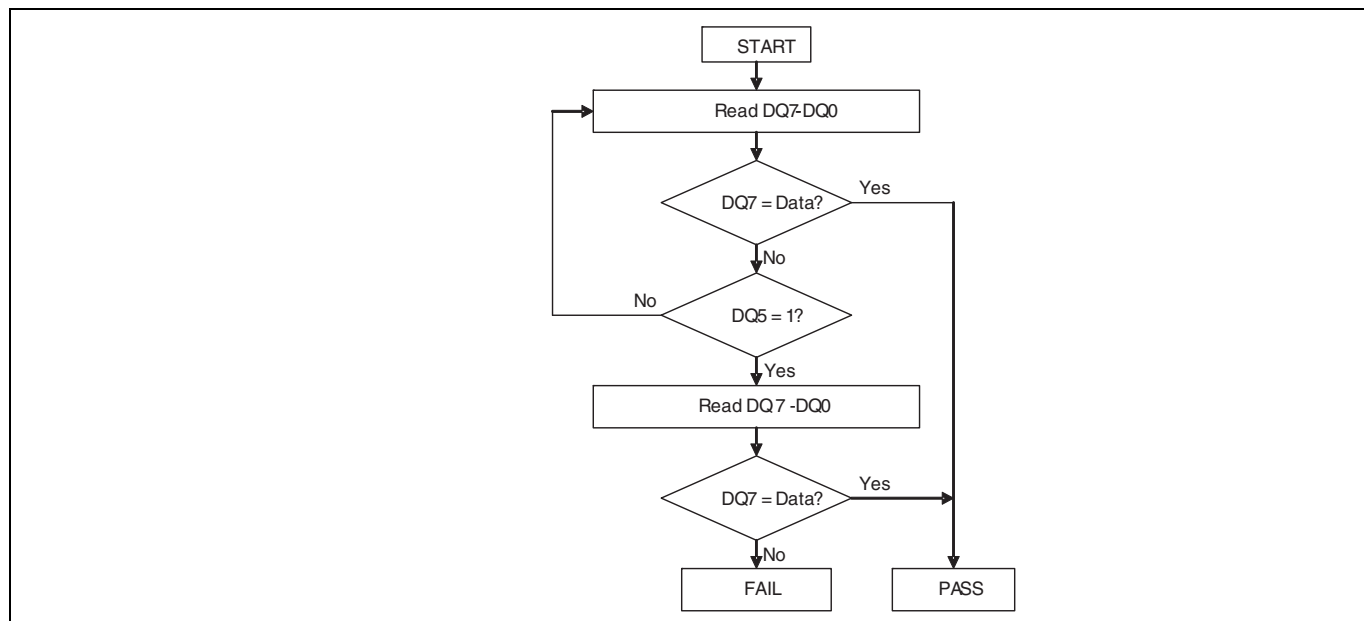
Figure 7 Data# Polling Algorithm [21]
