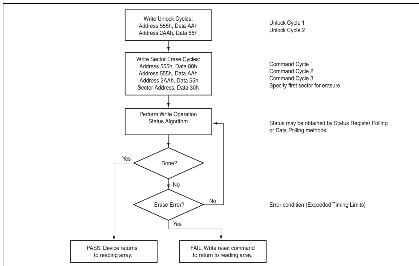
Figure 6 Sector erase operation
