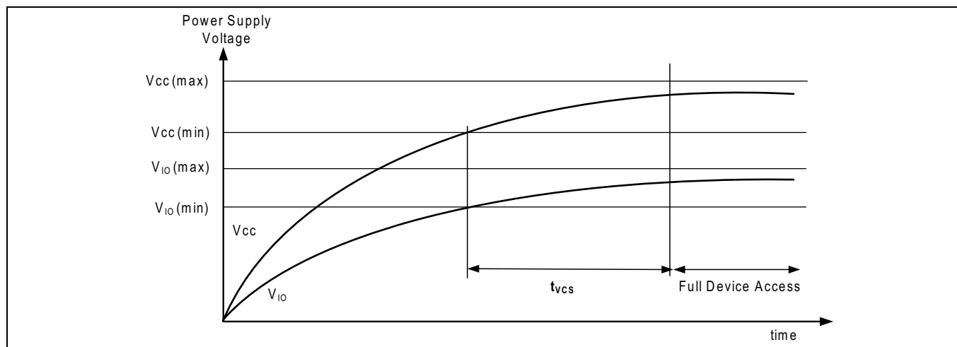
Figure 9 Power-up
