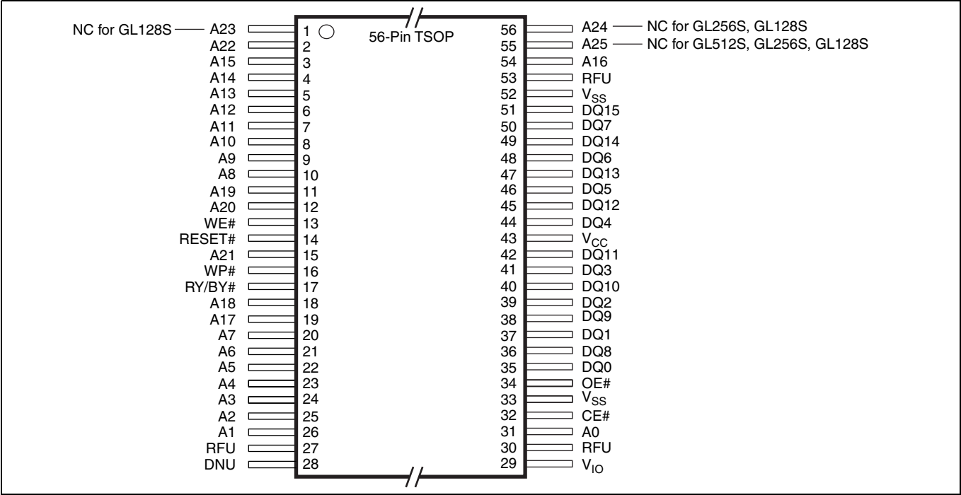
Figure 34 56-pin standard TSOP [105, 106]
