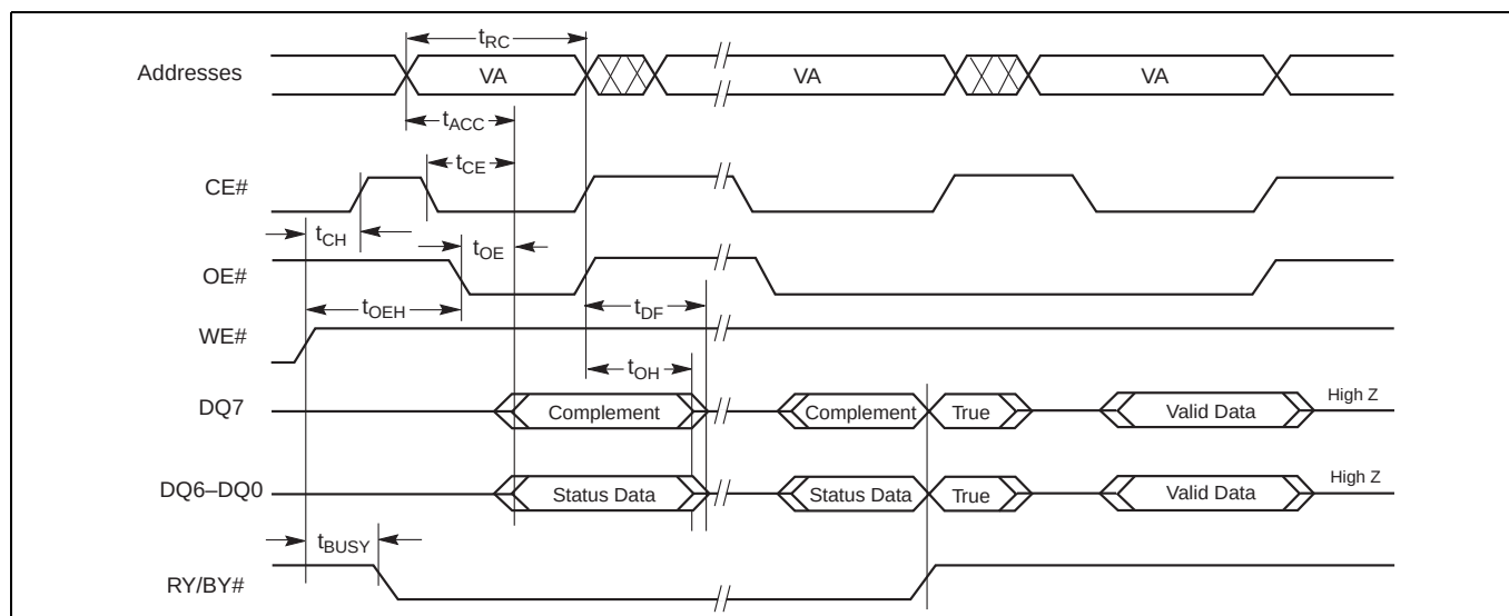
Figure 29 Data# Polling timing diagram (During Embedded Algorithms) [101]
