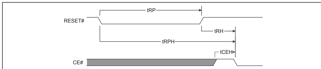
Figure 16 Hardware Reset
