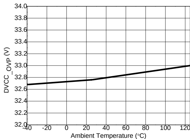
DVCC OVP Voltage vs. Ambient Temperature
