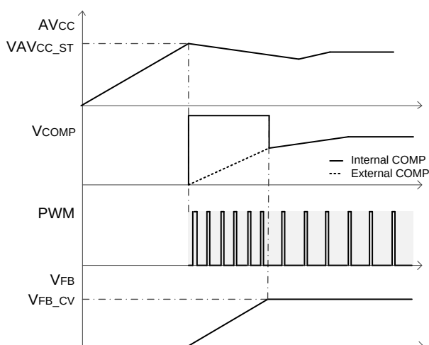
Figure 5. Start Up Waveform
