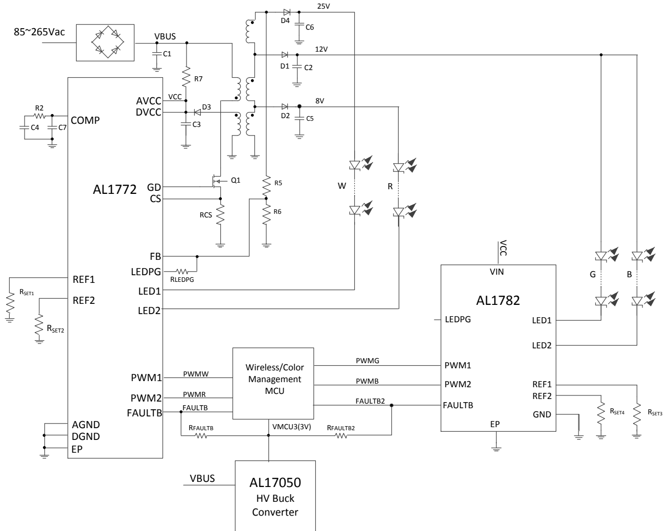
Figure 3. 4-Channel White+RGB
