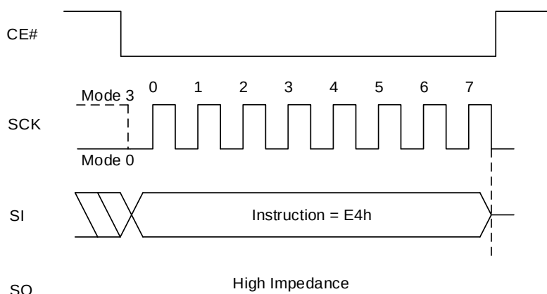
Figure 8.82 Erase PPB Sequence In SPI Mode
