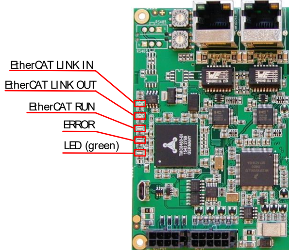
Figure 7.3: LEDs on TMC6213 interface brick
