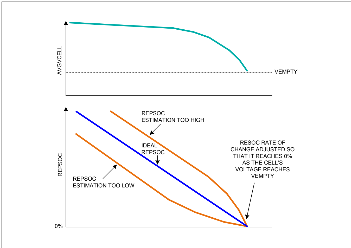
Figure 20. Converge-To-Empty
