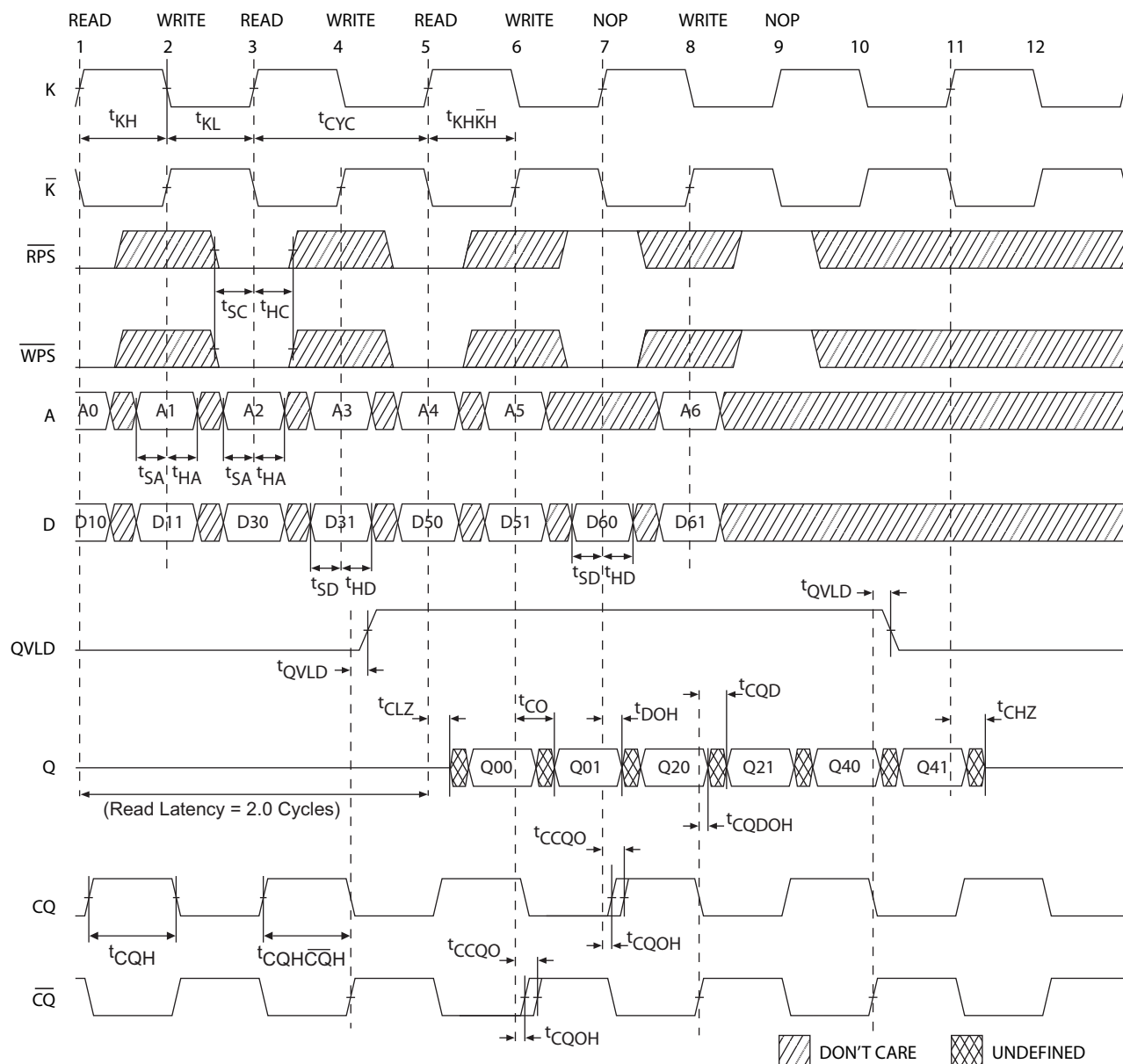
Figure 6. Waveform for 2.0 Cycle Read Latency [38, 39, 40]
