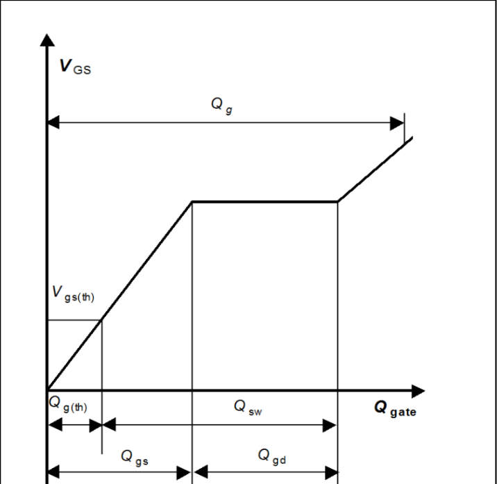
Diagram Gate charge waveforms
