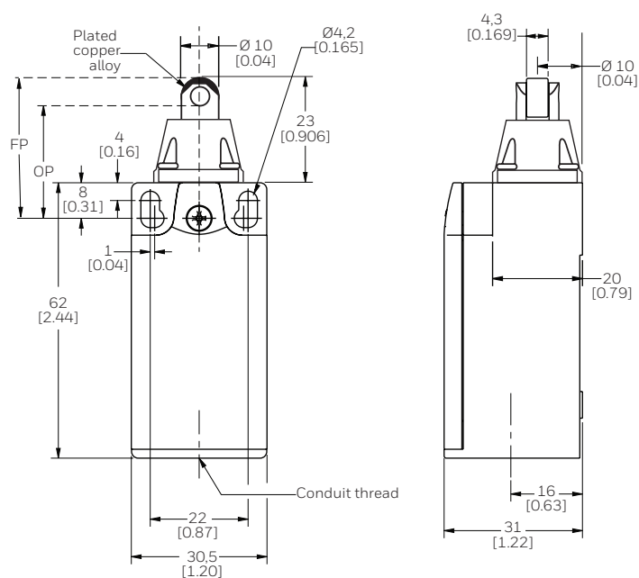
Figure 8. GLL Top Roller Plunger Dimensions
