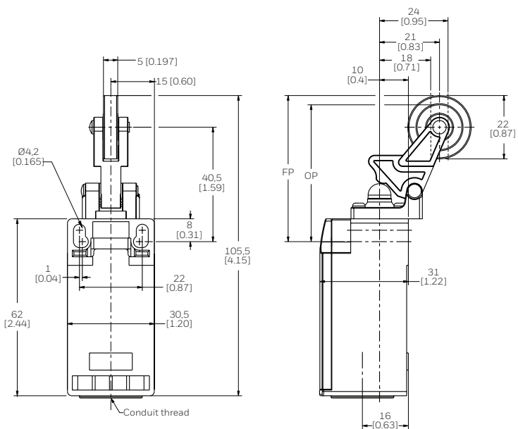
Figure 11. GLL Top Vertical Roller Lever Dimensions
