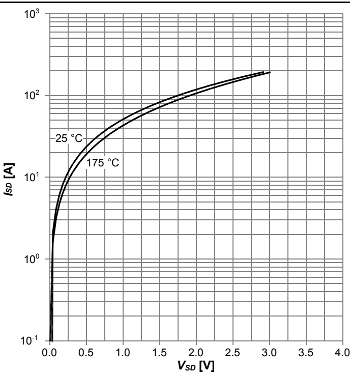
Diagram 12: Typ. reverse characteristics
