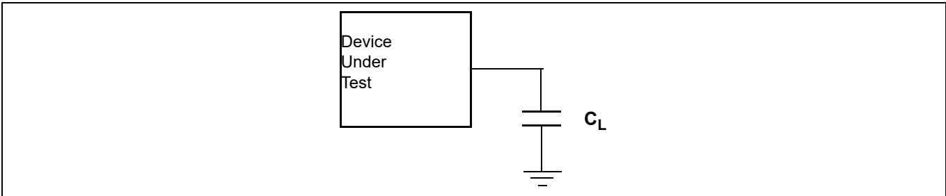
Figure 17 Test setup
