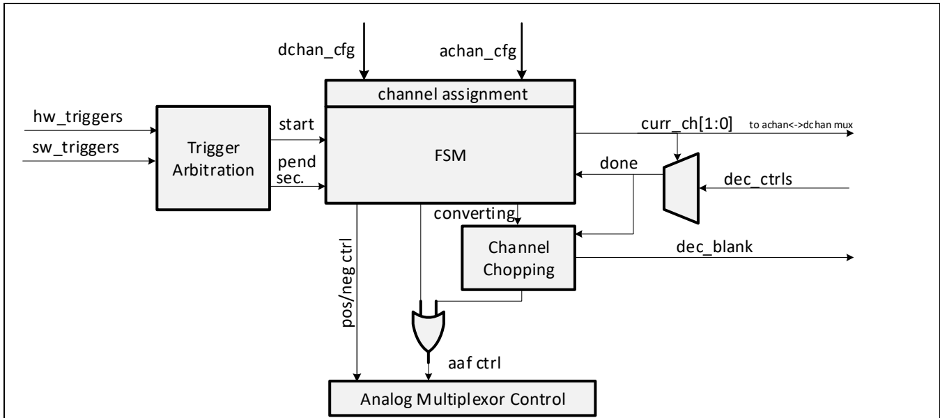
Figure 6 PACSS sequencer
