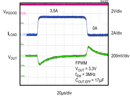
LOAD-TRANSIENT RESPONSE MAX20403AFLH
