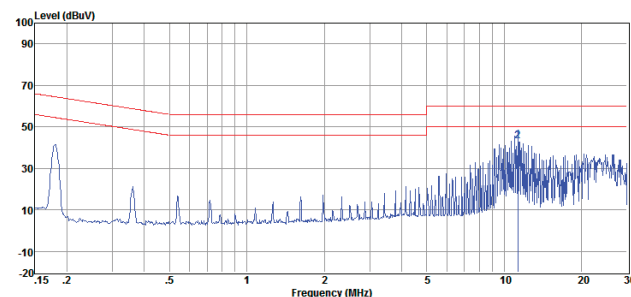
Graph 2. Conducted emissions performance, Negative Line, CISPR 22, Class B, full load
